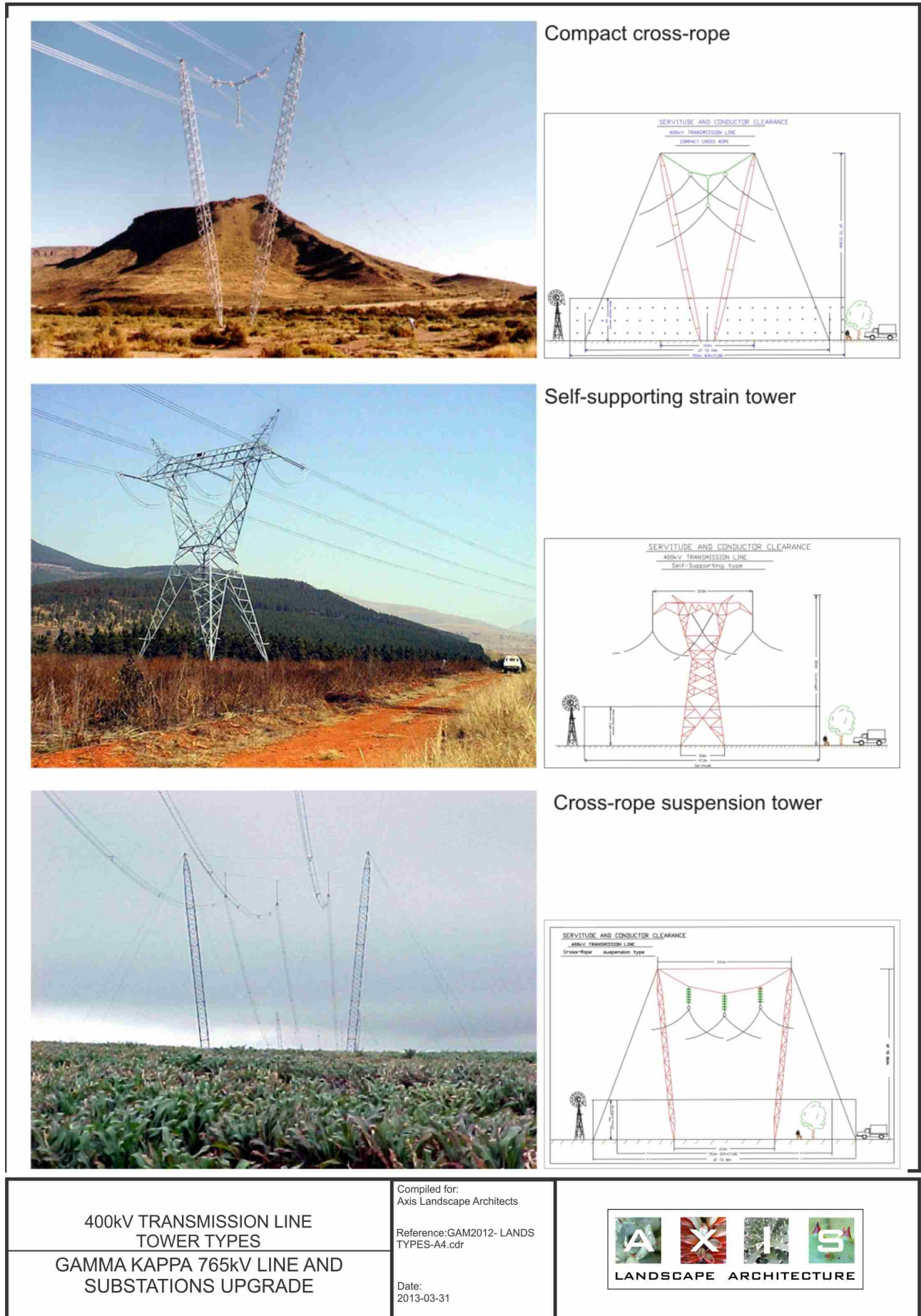
Figure 4: Tower Types
