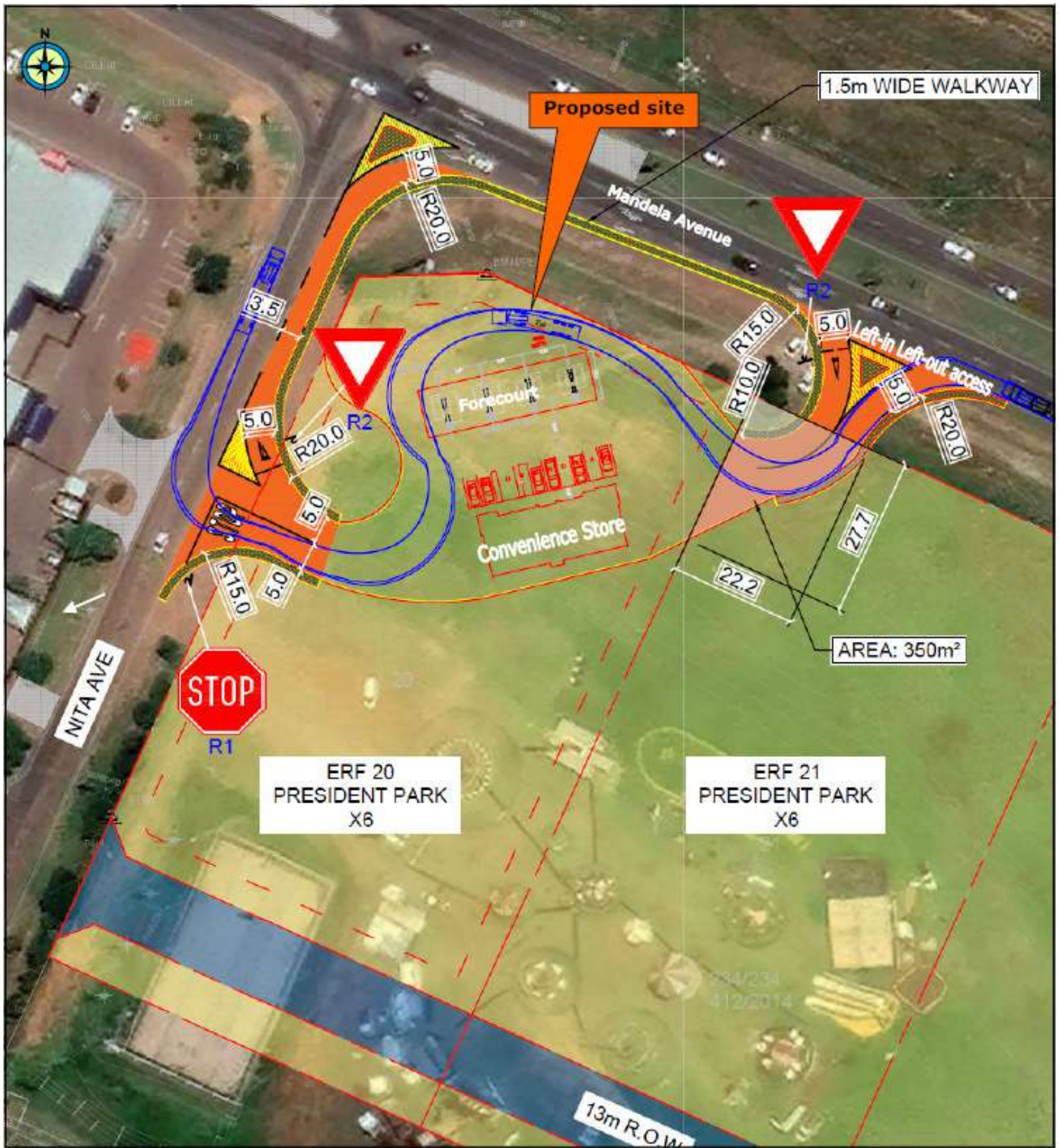
Figure 2: Site Development Plan (drafted by EDL Consulting Engineers, 2020)
