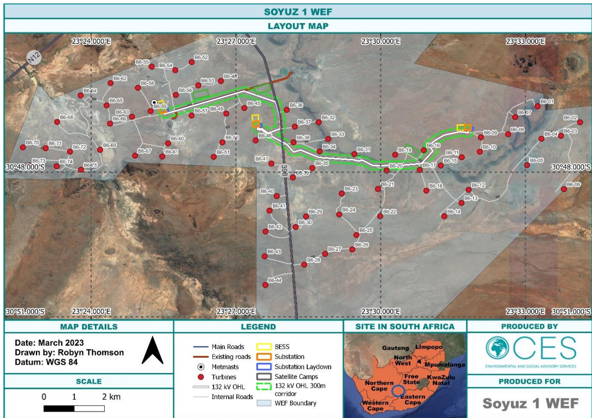
Figure 1: Layout Map of the Proposed Soyuz 1 WEF.
