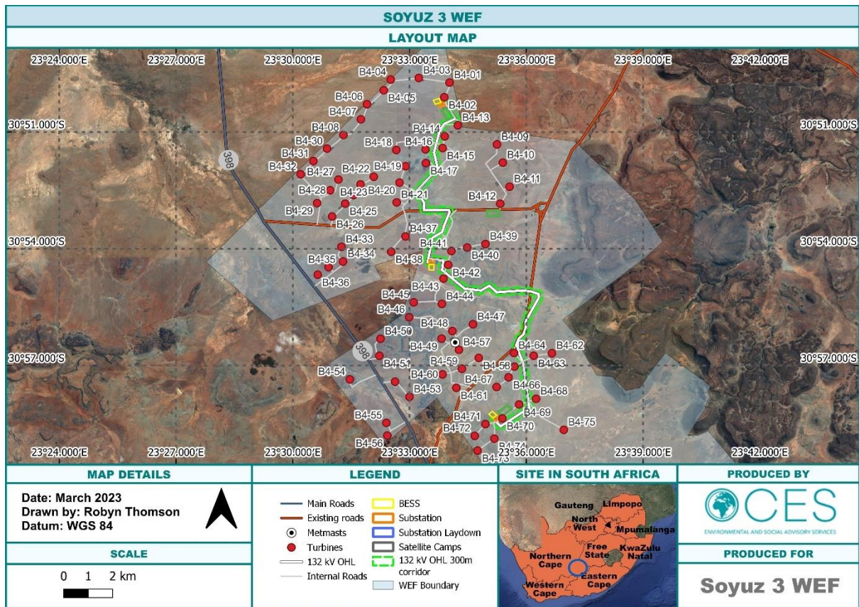
Figure 1: Layout Map of the Proposed Soyuz 3 WEF.
