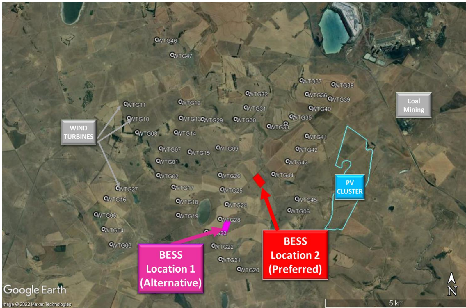
Figure 2.1.3 – Location of the BESS facilities within the site
