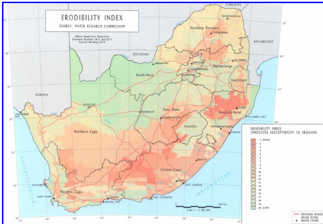
Figure 6: Erodibility Index
