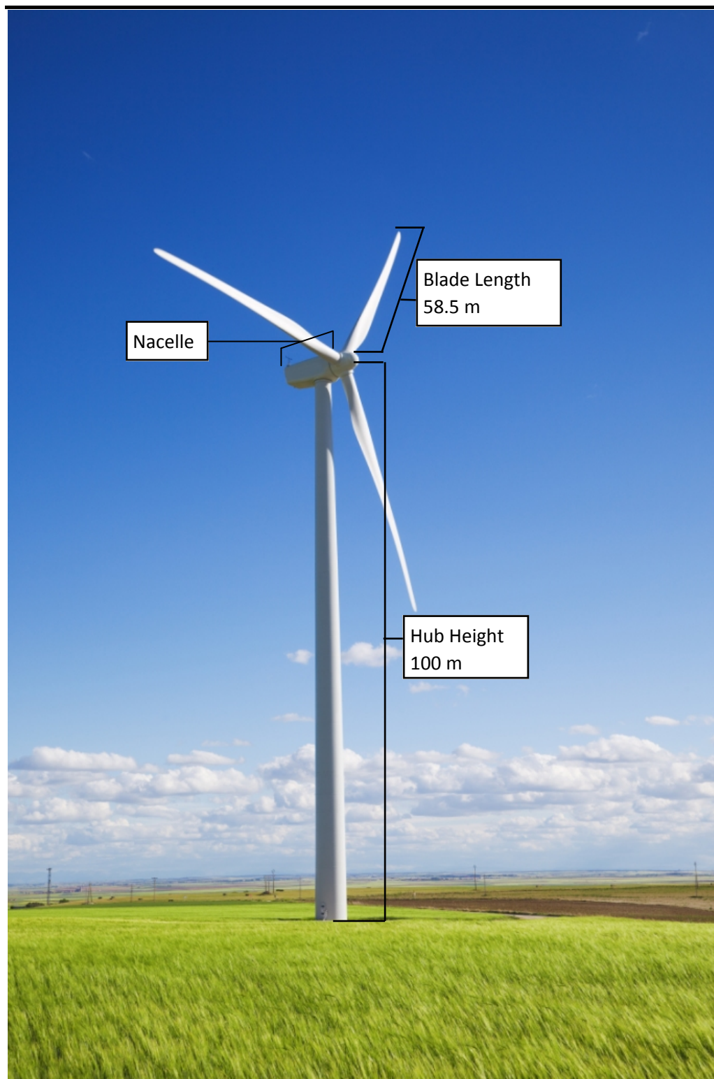
Figure 4.2 Typical Wind Turbine
