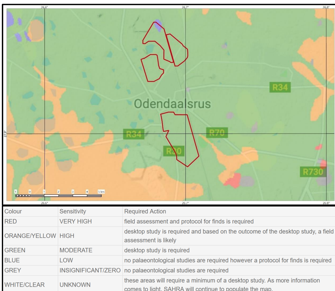
Figure 3. The Palaeontological sensitivity of the project area
