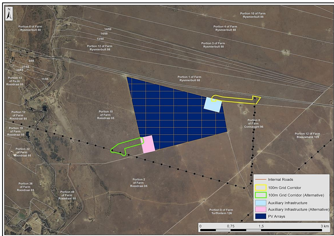
Figure 5.3: Draft layout plan for the Rooidraai solar PV facility and proposed grid alternatives
