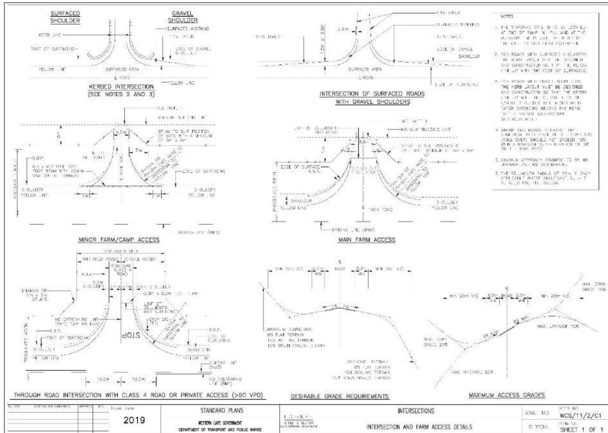
Figure 7.7 Typical Intersection and Farm Access Detail
