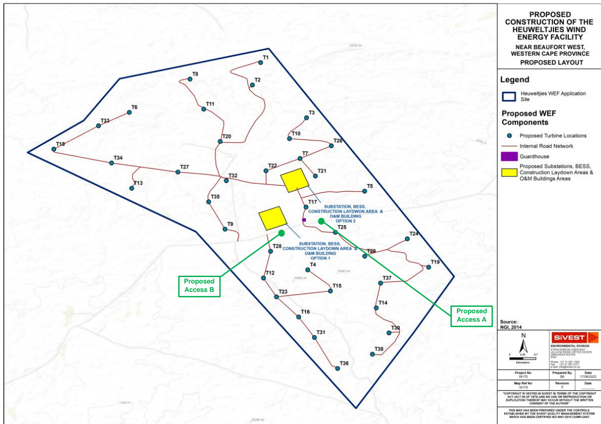
Figure 8.1 Heuweltjies WEF - Internal Layouts and proposed access points
