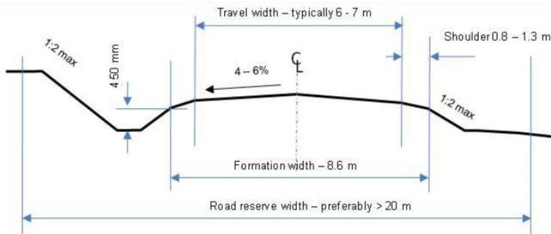
Figure 7.9 Typical Provincial Gravel Road Cross Section
