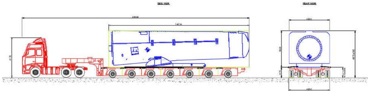
Figure 7.1 Example of Nacelle
