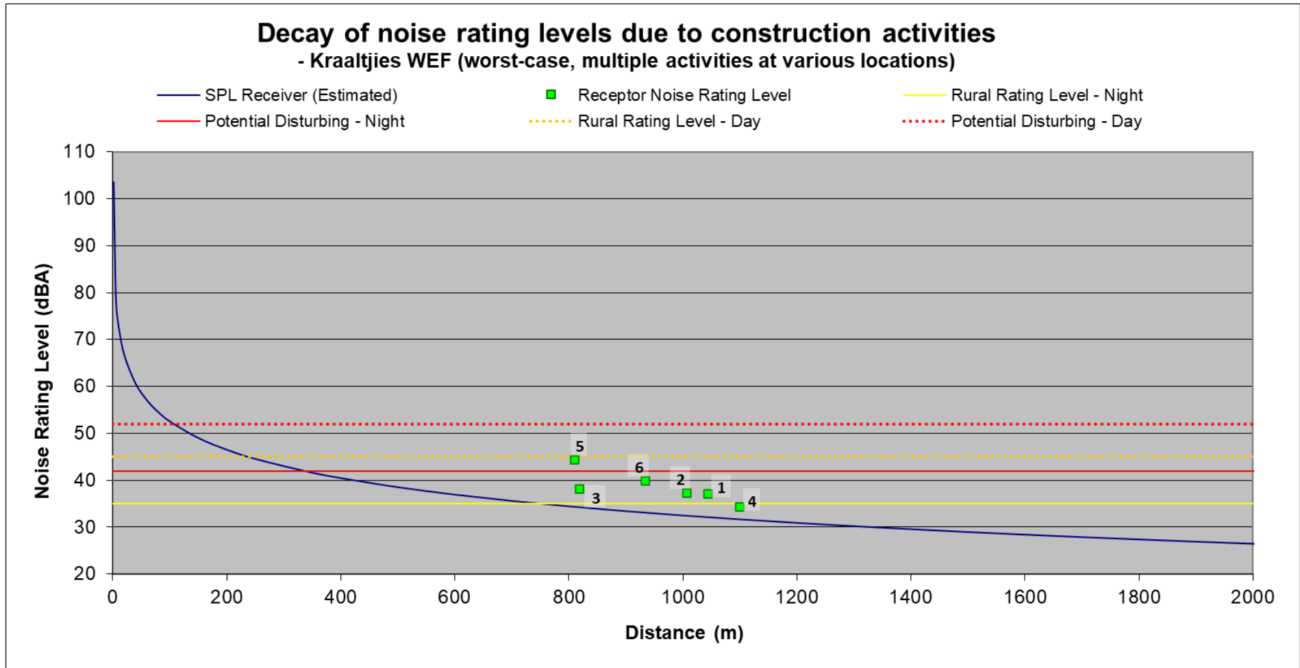
Figure 9-3: Projected conceptual construction noise levels for the proposed Kraaltjies WEF
