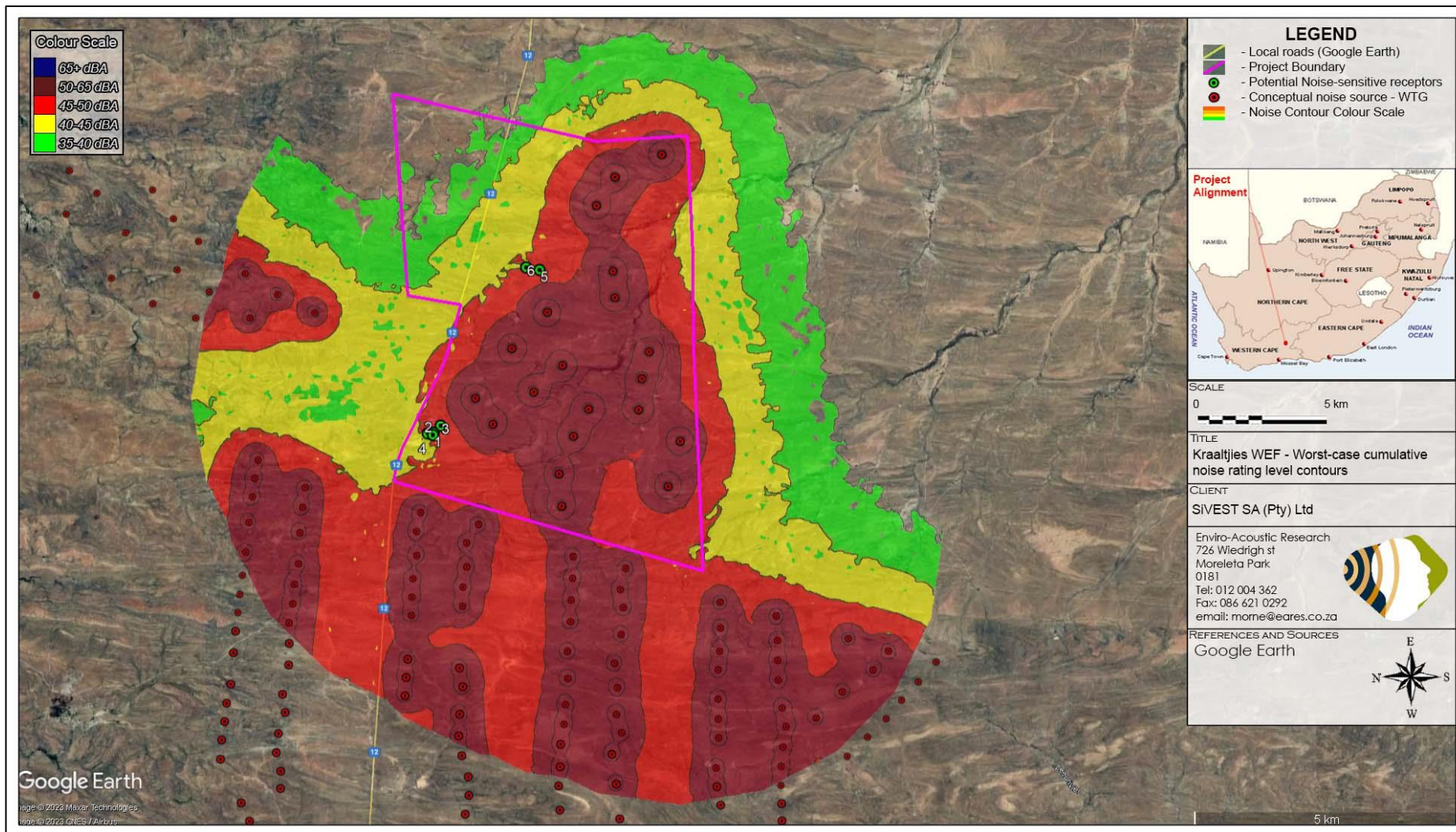
Figure 9-7: Projected future cumulative noise rating level contours (worst-case SPL of 112.6 dBA re 1 pW)
