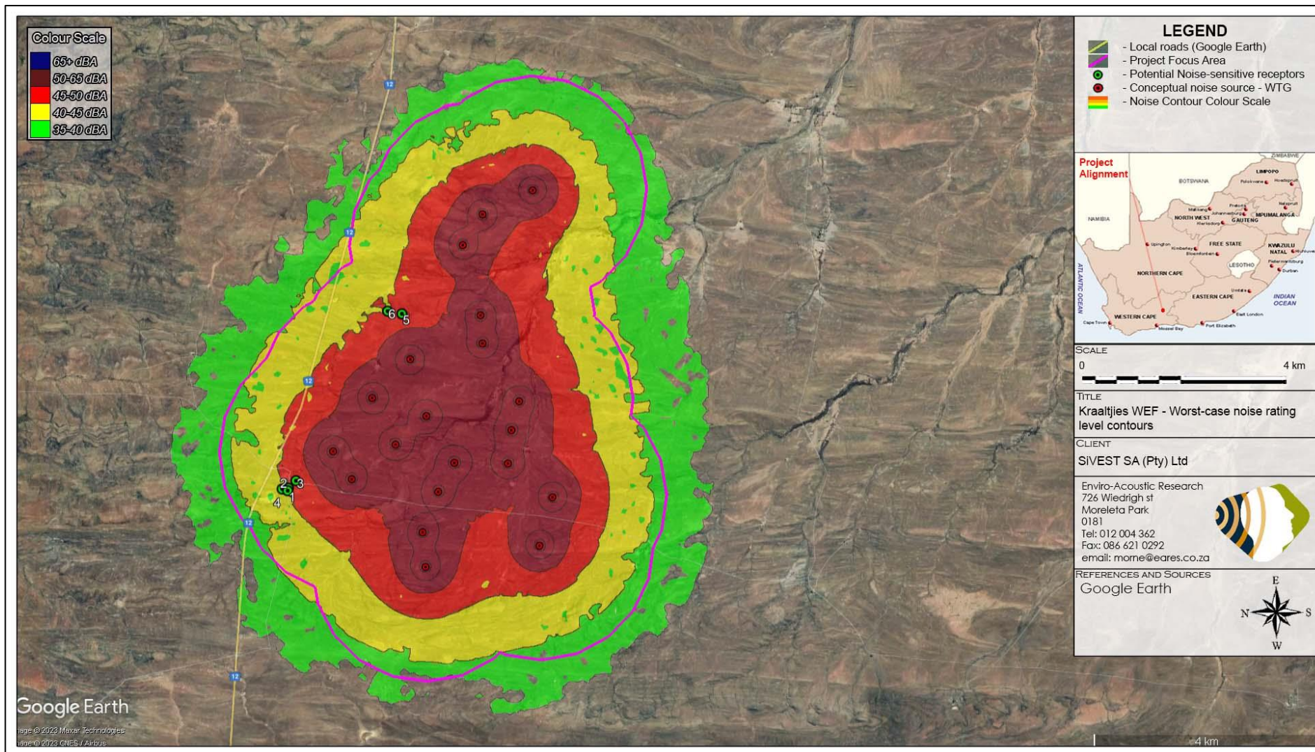
Figure 9-4: Projected future noise rating level contours (worst-case WTG with SPL of 112.6 dBA re 1 pW)
