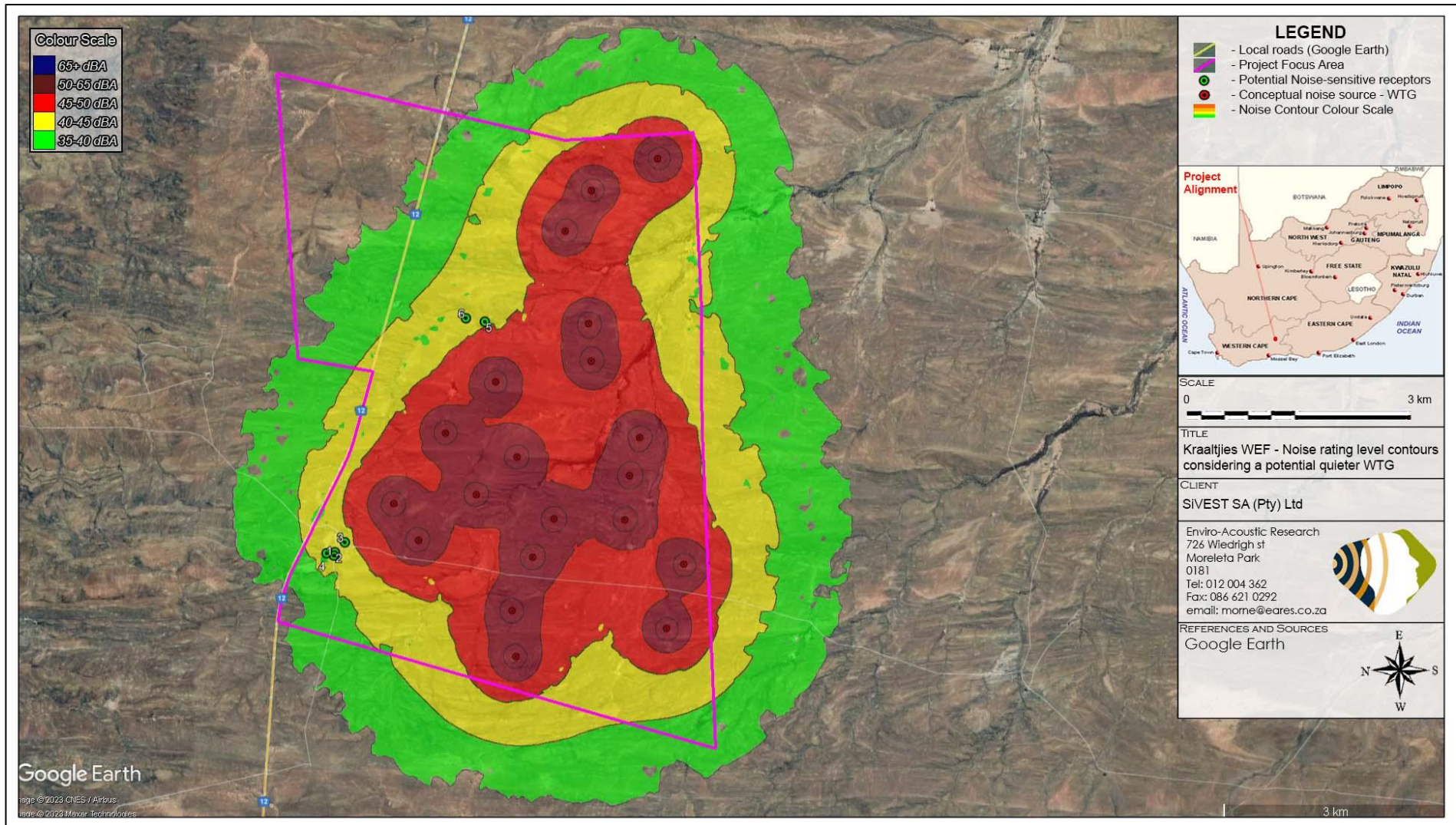
Figure 9-5: Projected future noise rating level contours (WTG with SPL of 109.5 dBA re 1 pW)
