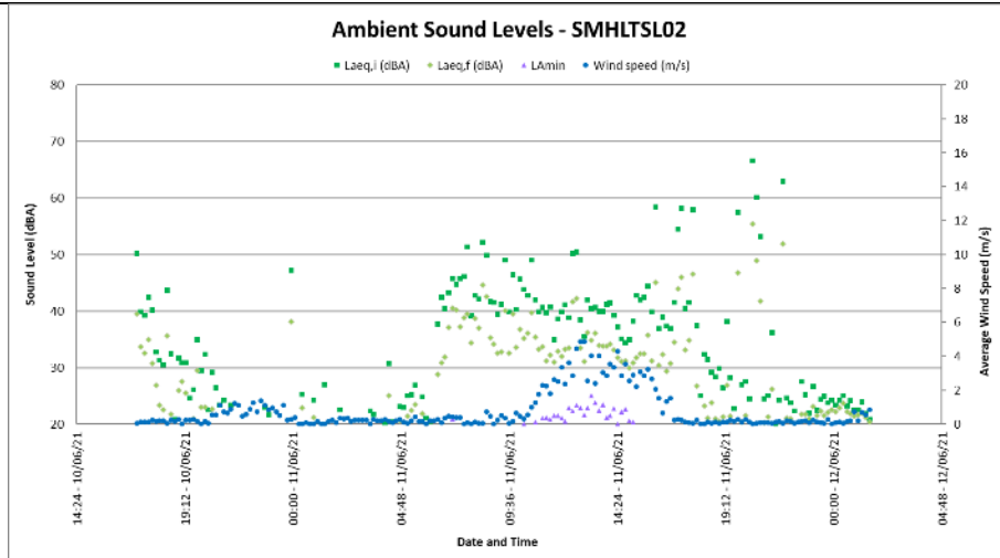
Figure 4-29: Ambient Sound Levels at SMHLTSL02
