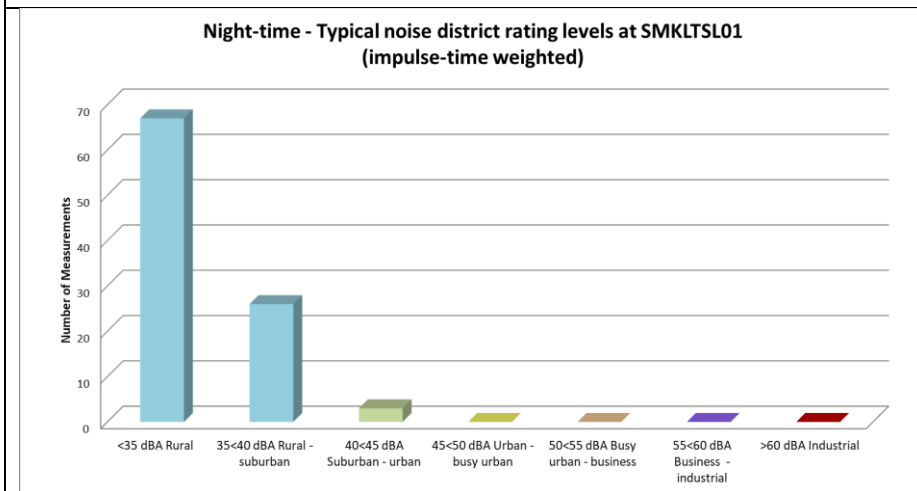
Figure 4-19: Classification of night-time measurements in typical noise districts at SMKLTSL01
