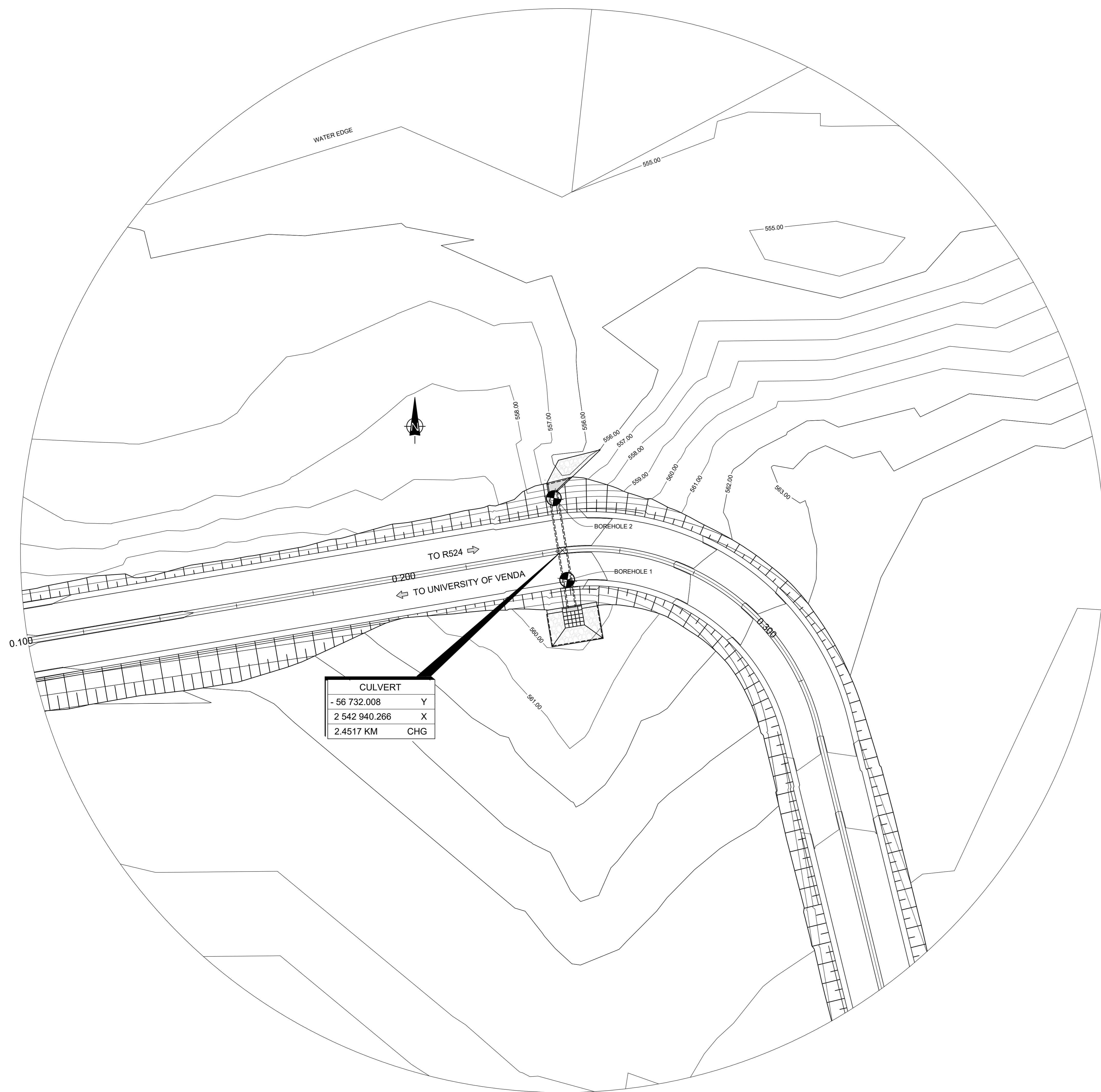
CULVERT - SITE PLAN SCALE 1:500
