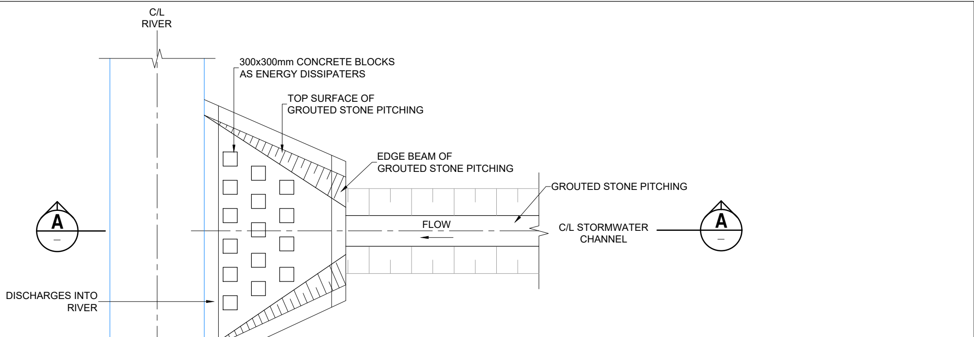
TYPICAL PLAN OF ENERGY DISSIPATER
