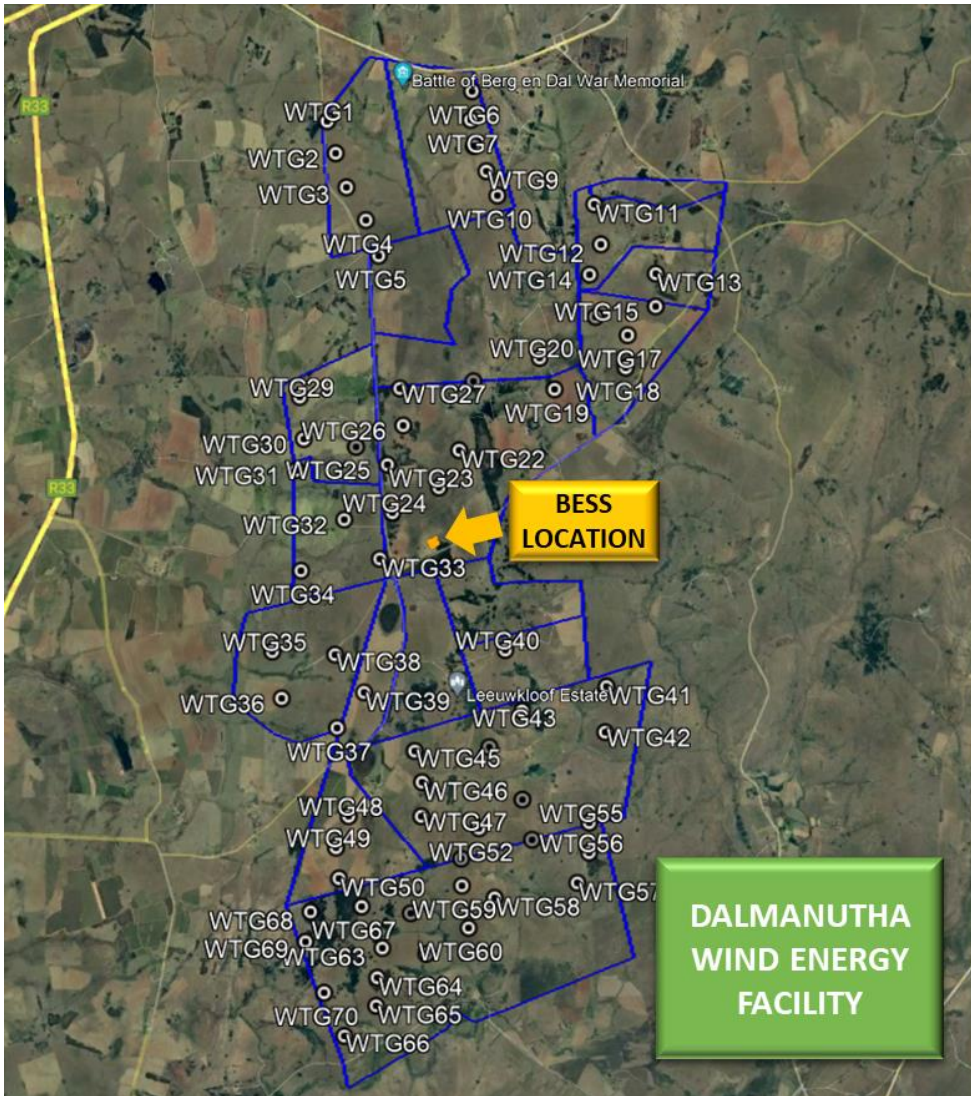
Figure 2.1.3 - The layout of the system for the two options WEF or Hybrid WEF & SEF showing the same location of interest for the BESS
