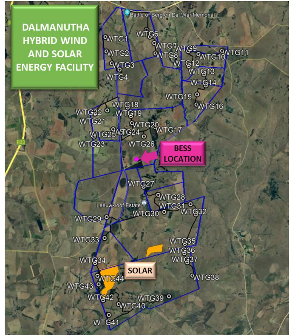
Figure 2.1.3 - The layout of the system for the two options WEF or Hybrid WEF & SEF showing the same location of interest for the BESS
