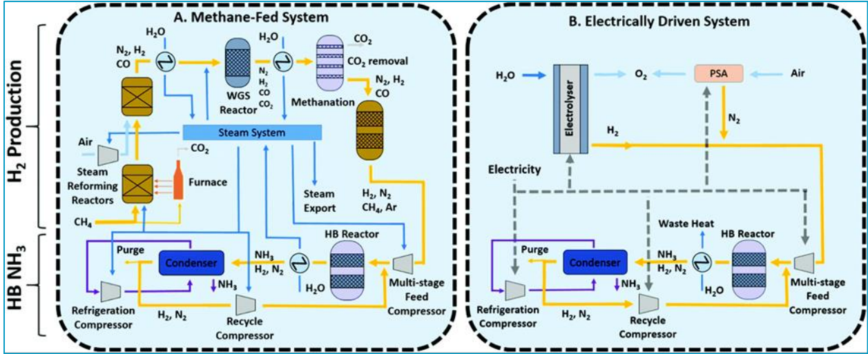
Figure 1.2: Green Hydrogen and Ammonia Production - Simplified Process Flow Diagram.
