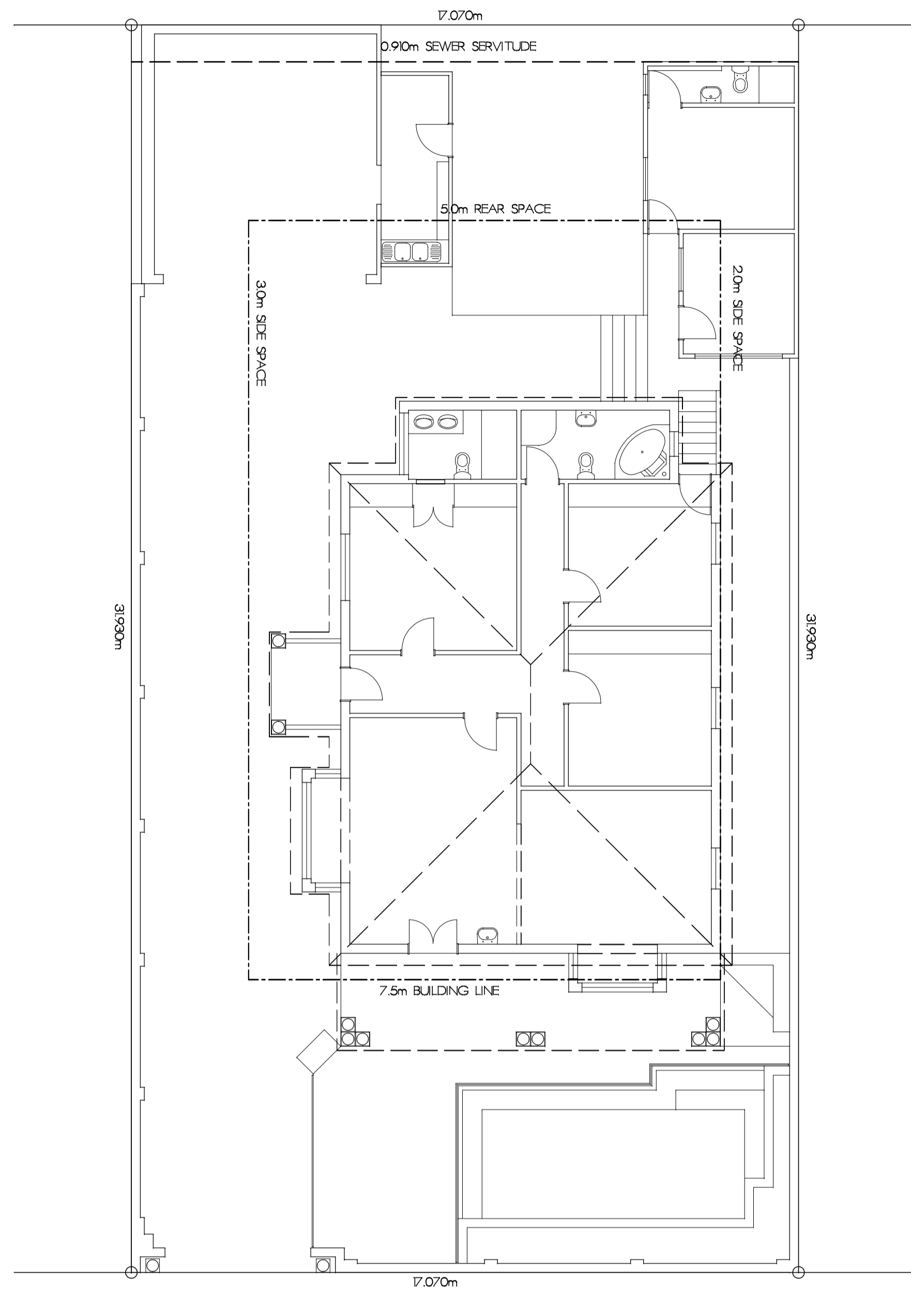
NELSON ROAD GROUND STOREY & SITEPLAN SCALE 1/100
