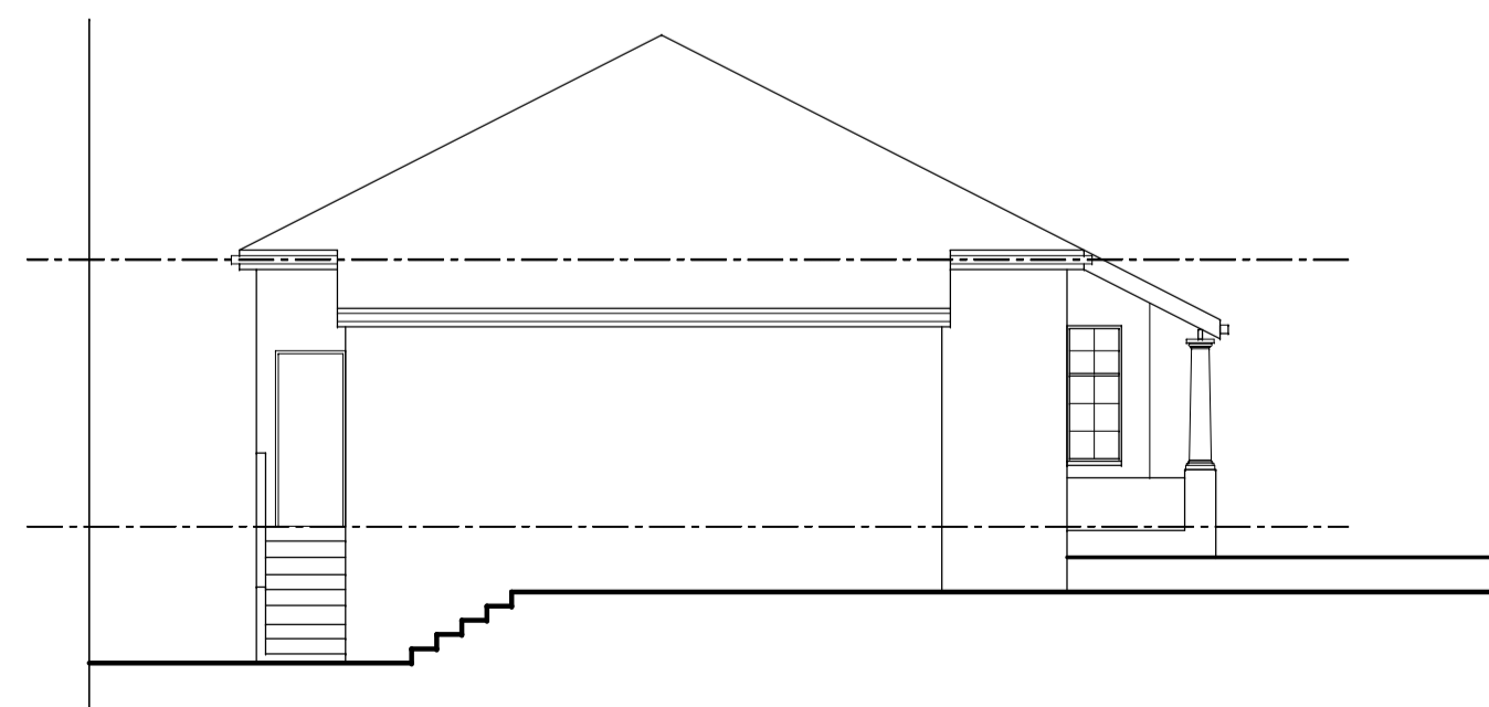
SW ELEVATION SCALE 1/100
