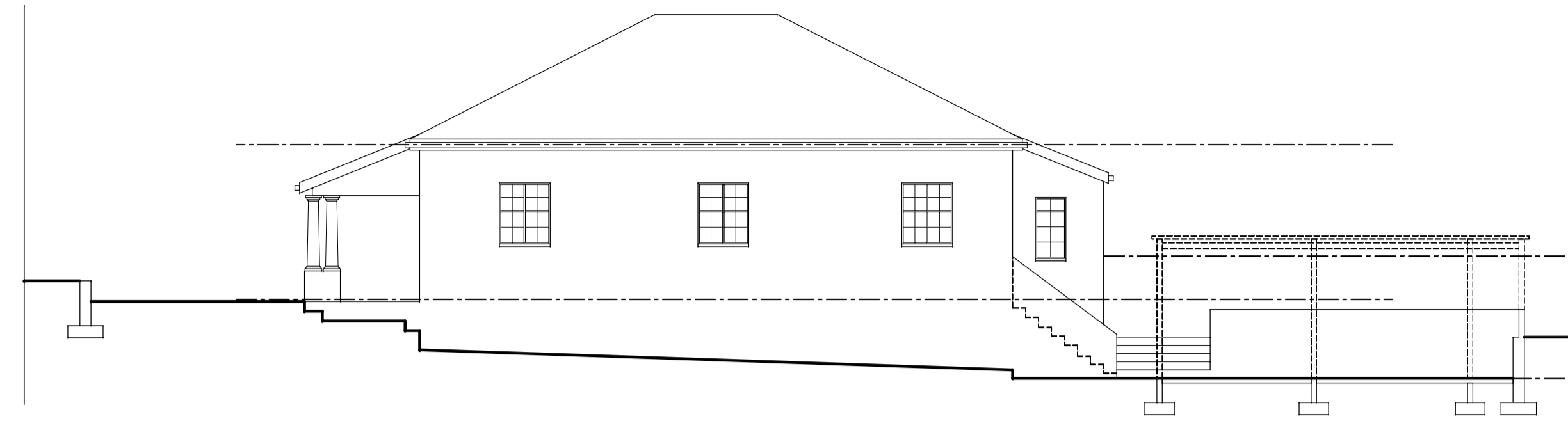
NW ELEVATION SCALE 1/100
