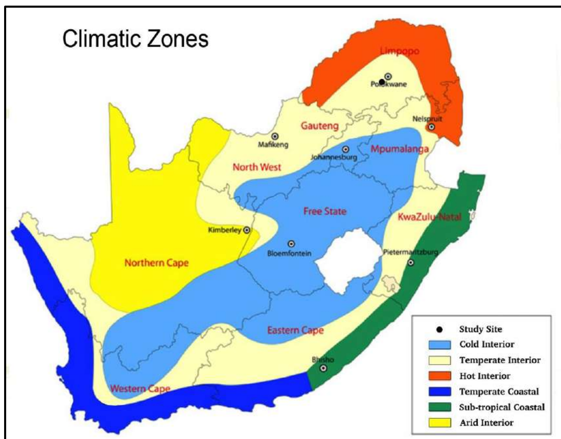
Figure 4: Climatic Regions of South Africa
