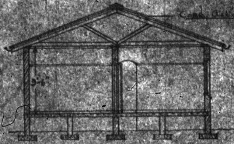
SECTION AD
