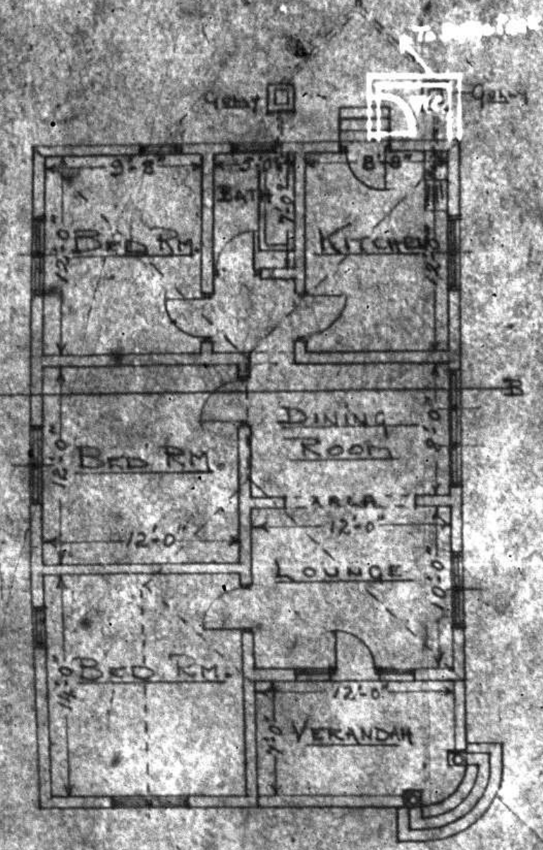
FLOOR PLAN
