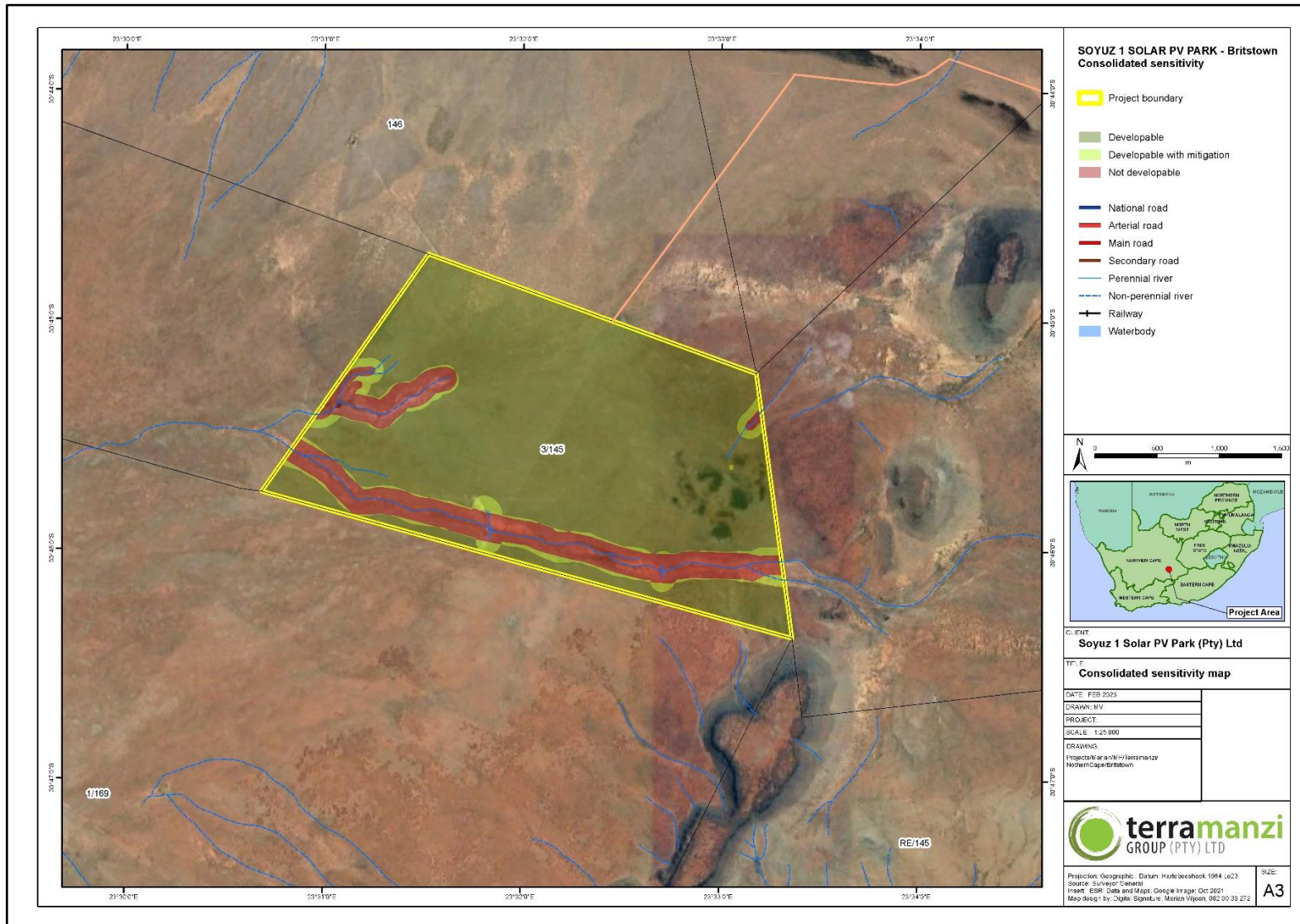
Figure 5: Site Map for the Soyuz 1 Solar PV Park showing the location of the Substation (dark green)
