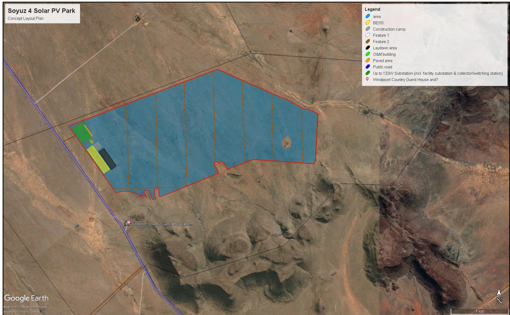
Figure 4: Site Map for the Soyuz 4 Solar PV Park showing the location of the Substation (dark green)
