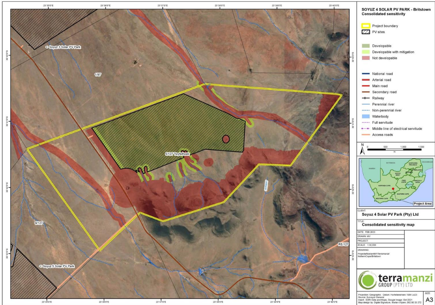
Figure 5: Site Map for the Soyuz 4 Solar PV Park showing the location of the Substation (dark green)
