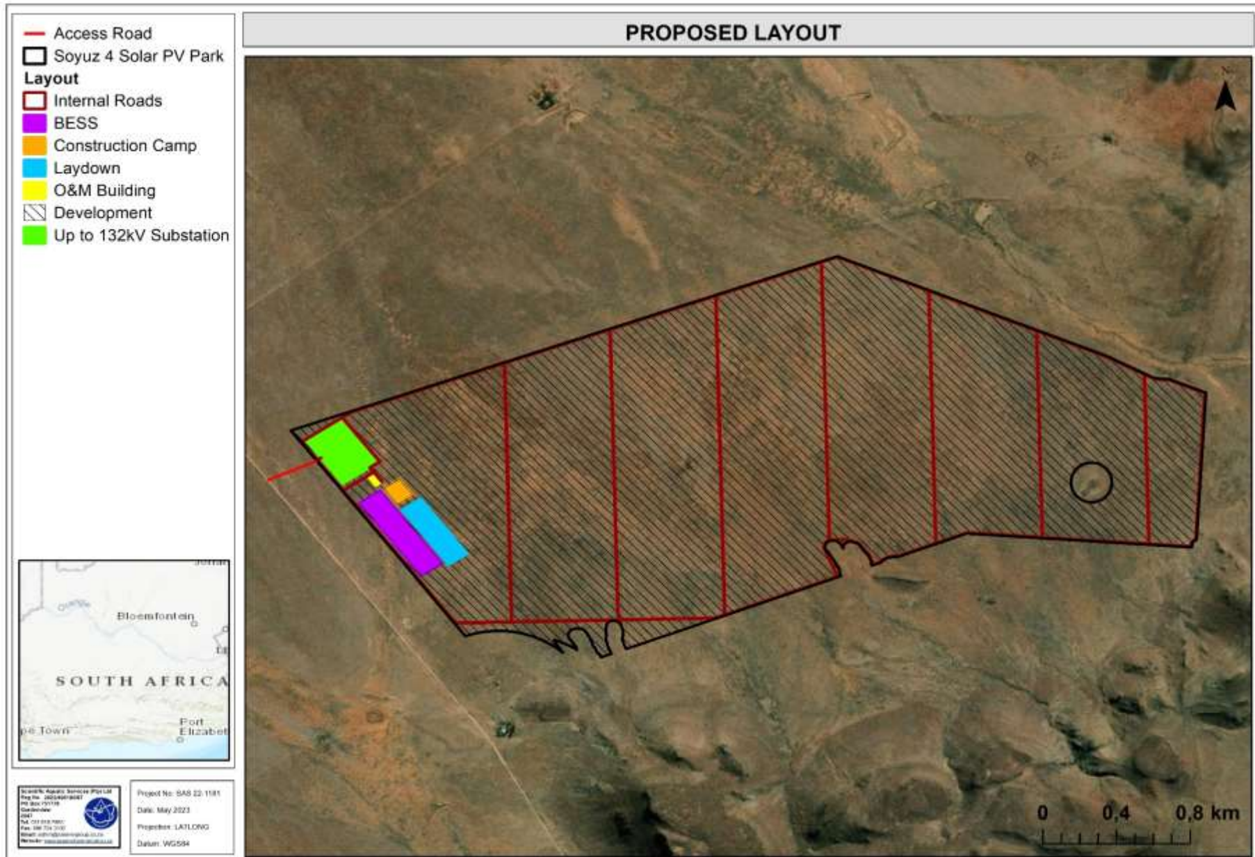
Figure 5: Proposed layout of the Soyuz 4 Solar PV Park.
