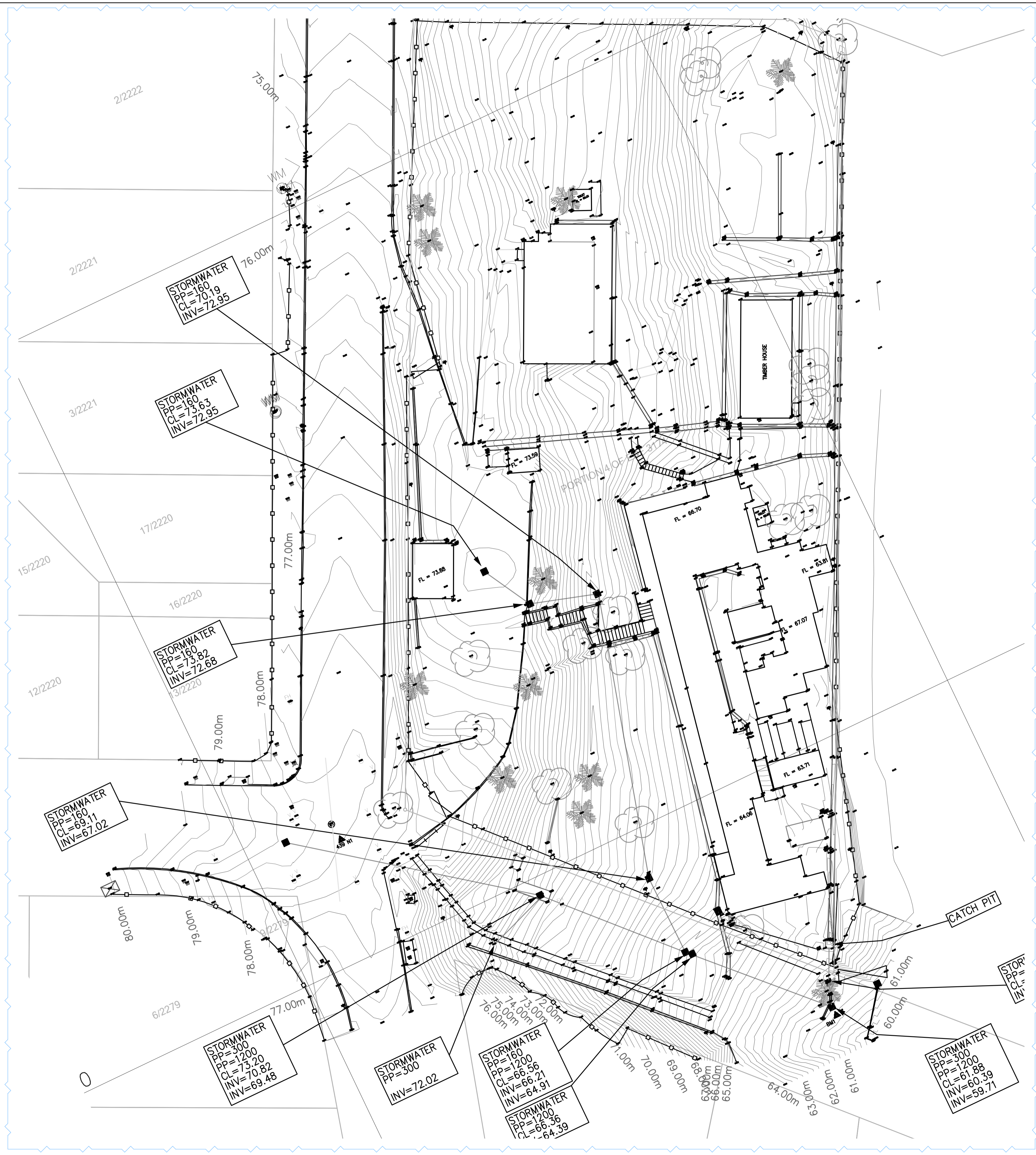
EXISTING SITE PLAN Scale:1:300
