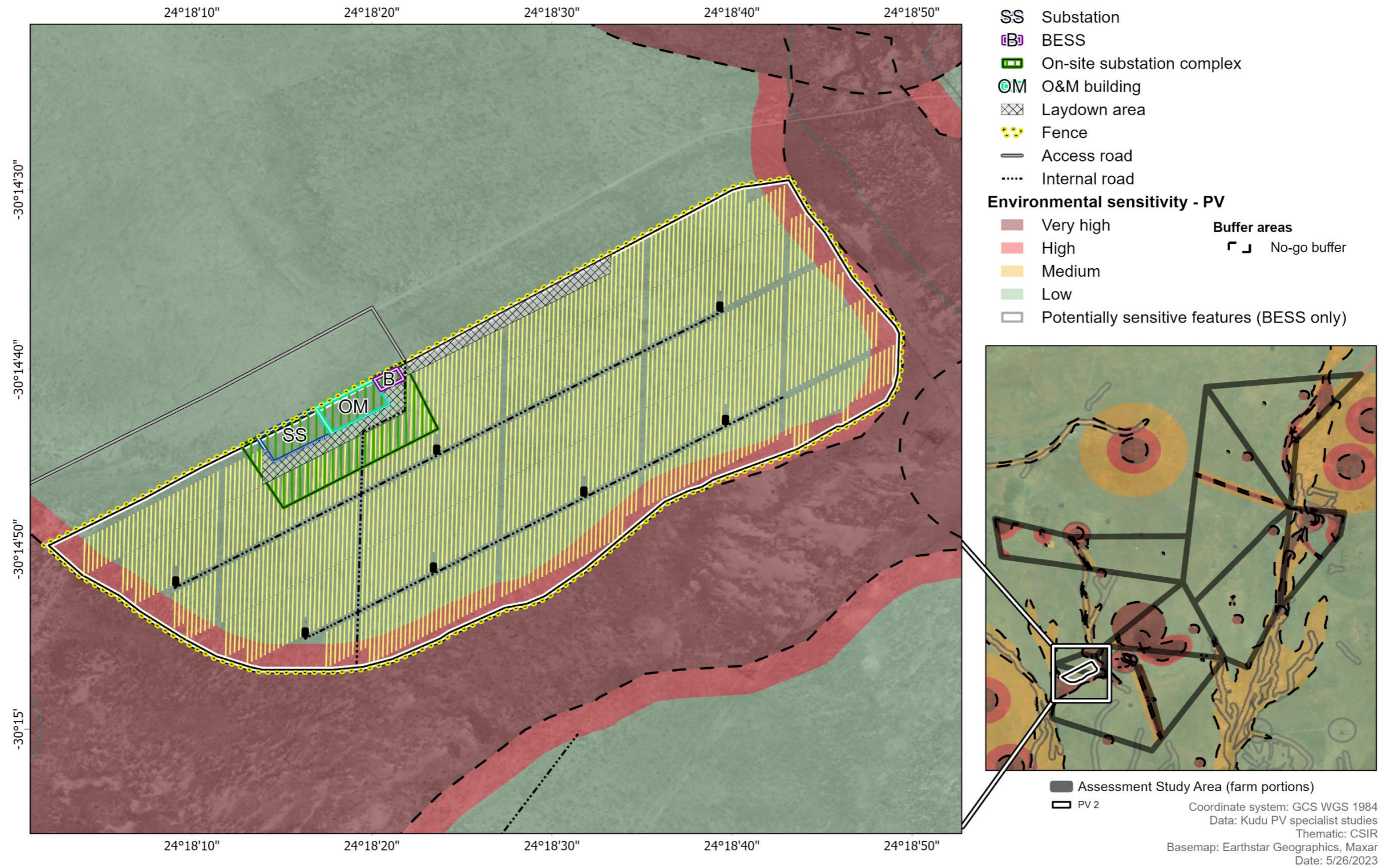
Combined Project Layout and Sensitivity Map.
