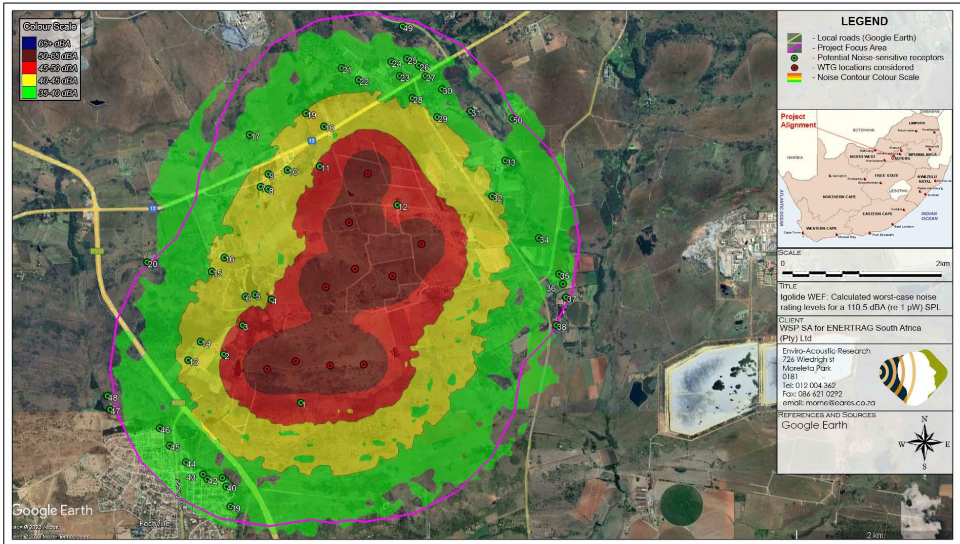
Figure 9-5: Projected future noise rating level contours (using an SPL of 109.0 dBA re 1 pW)
