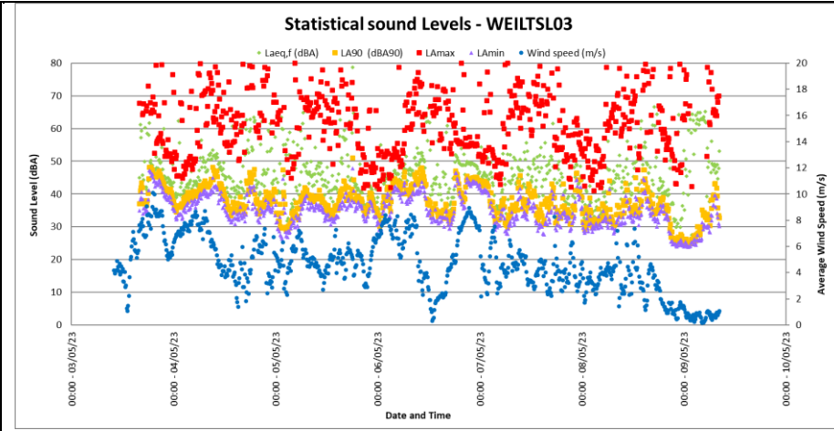
Figure 4-13: Maximum, minimum and Statistical sound levels at WEILTSL03
