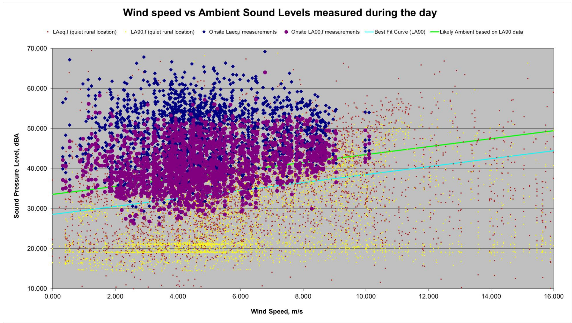
Figure 4-20: Daytime ambient sound levels measured in vicinity of project
