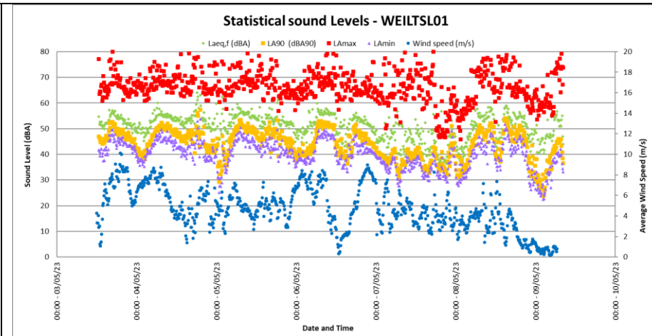
Figure 4-5: Maximum, minimum and Statistical sound levels at WEILTSL01
