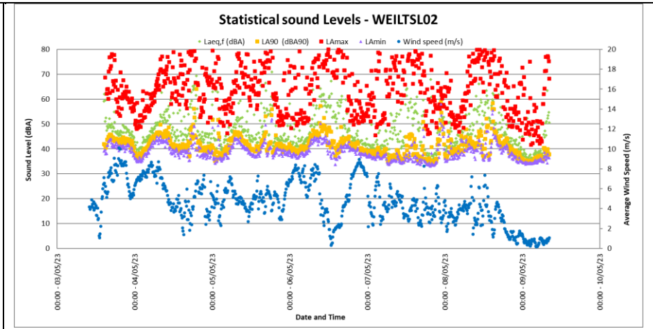
Figure 4-9: Maximum, minimum and statistical values at WEILTSLO2
