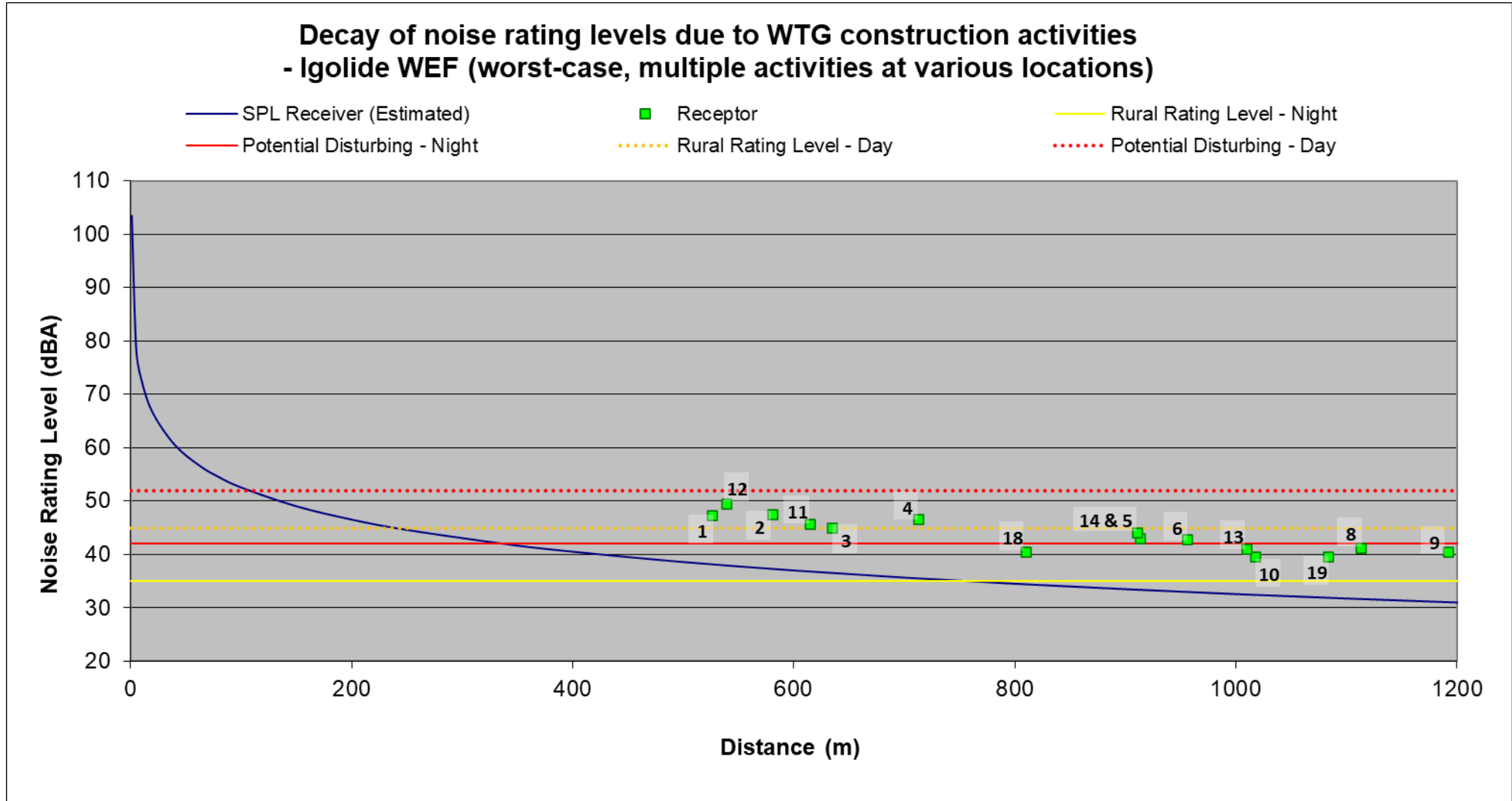
Figure 9-3: Projected conceptual construction noise levels for the proposed Igolide WEF
