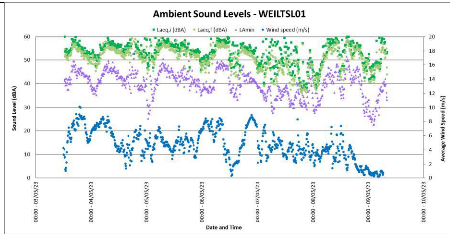
Figure 4-4: Ambient Sound Levels at WEILTSL01
