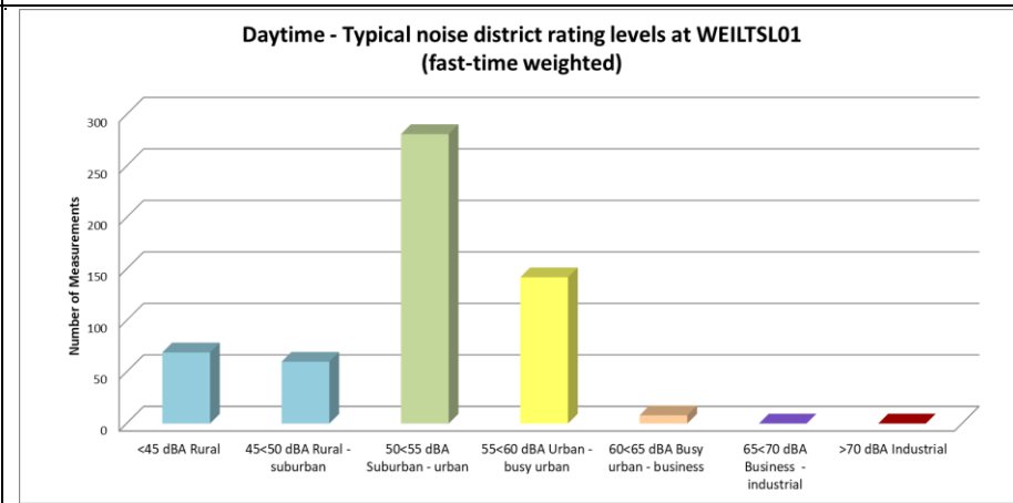
Figure 4-7: Classification of daytime measurements in typical noise districts at WEILTSL01
