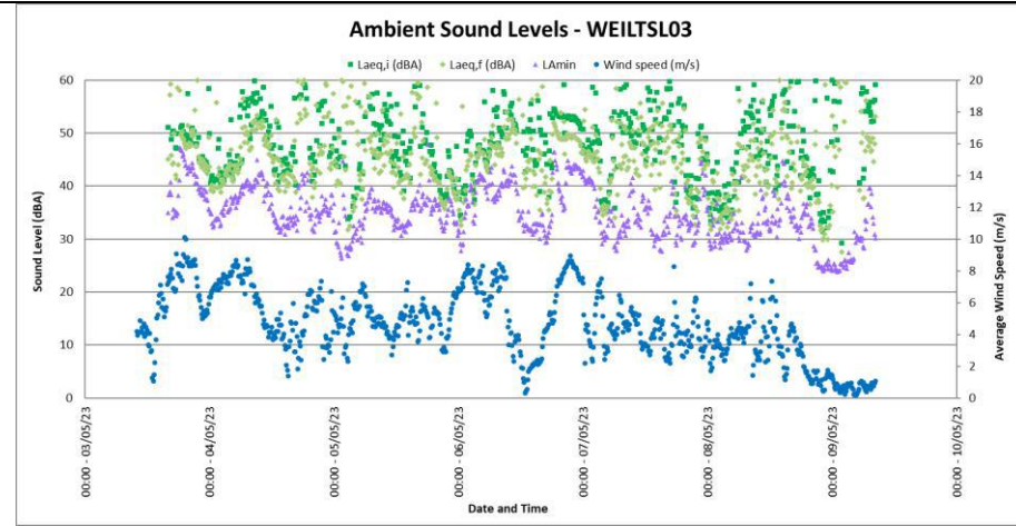
Figure 4-12: Ambient Sound Levels at WEILTSL03
