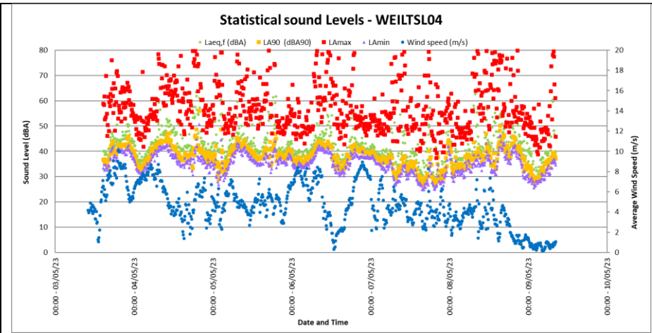
Figure 4-17: Maximum, minimum and Statistical sound levels at WEILTSLO4
