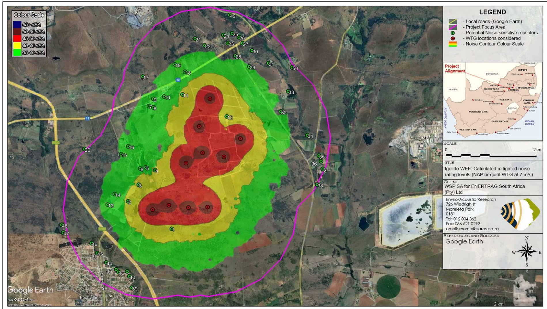
Figure 9-6: Projected future noise rating level contours (use of NAP or quieter WTG at a 7m/s wind)
