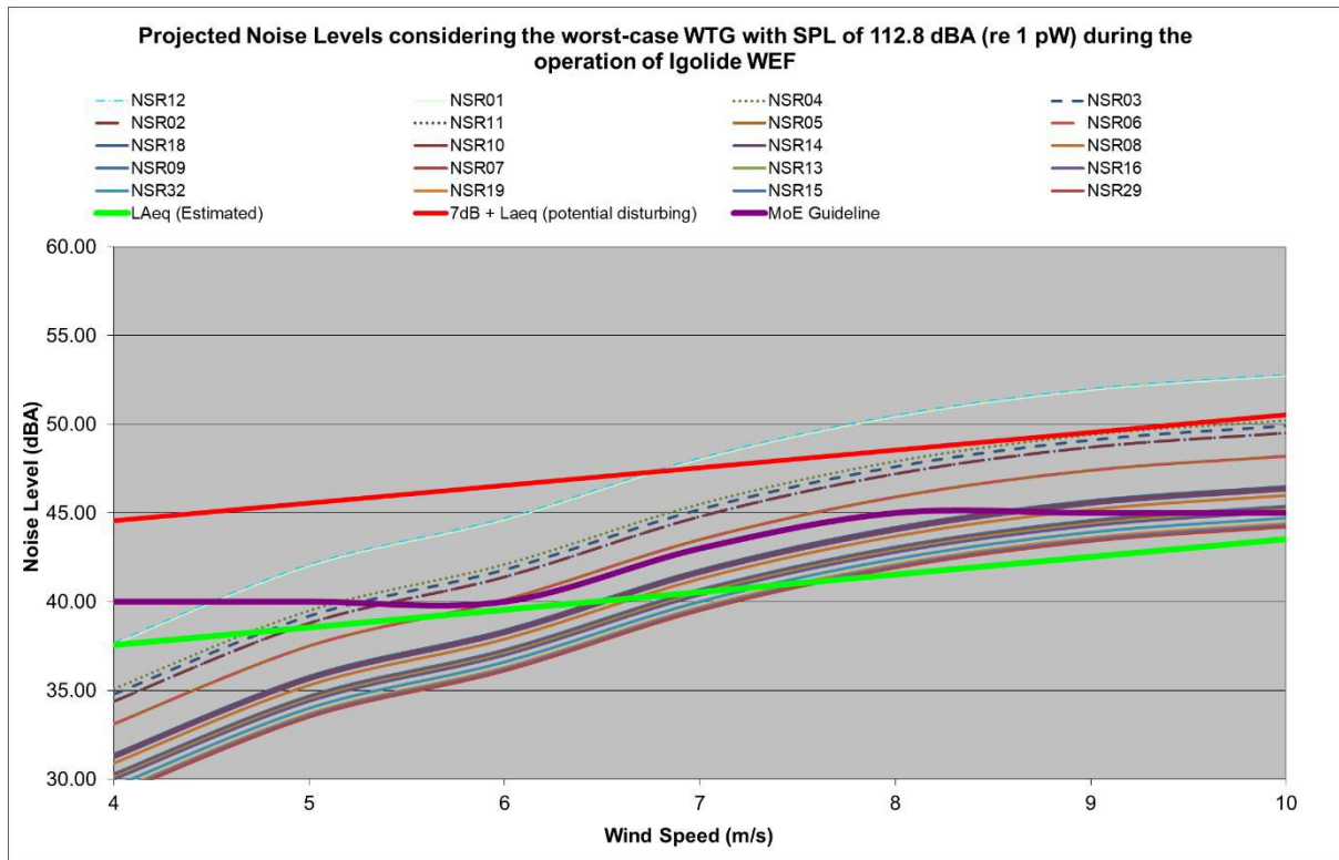
Figure 9-4: Projected noise levels at different wind speeds
