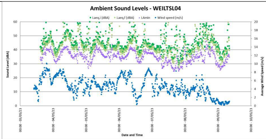
Figure 4-16: Ambient Sound Levels at WEILTSLO4
