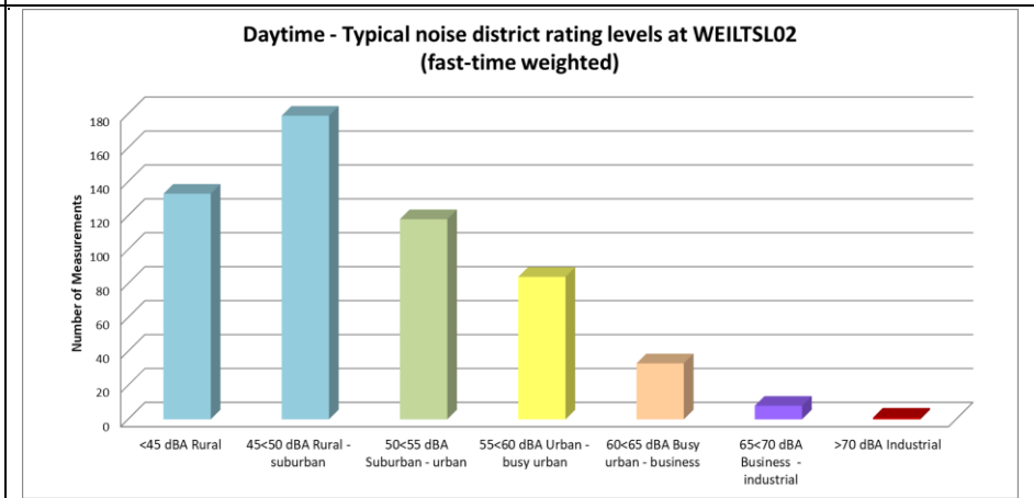
Figure 4-11: Classification of daytime measurements in typical noise districts at WEILTSLO2
