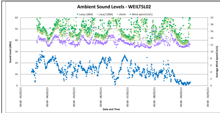
Figure 4-8: Ambient sound levels at WEILTSLO2
