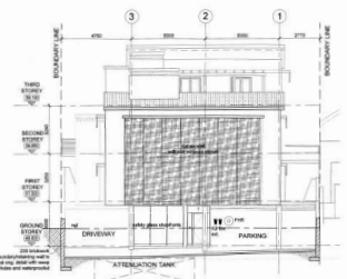
SOUTH EAST ELEVATION TO PROBLEM MKHIZE ROAD (without fence)
