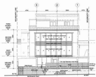
SOUTH EAST ELEVATION FROM PROBLEM MKHIZE ROAD (with fence)
