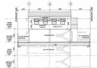
NORTH WEST ELEVATION TO ELEVENTH AVE
