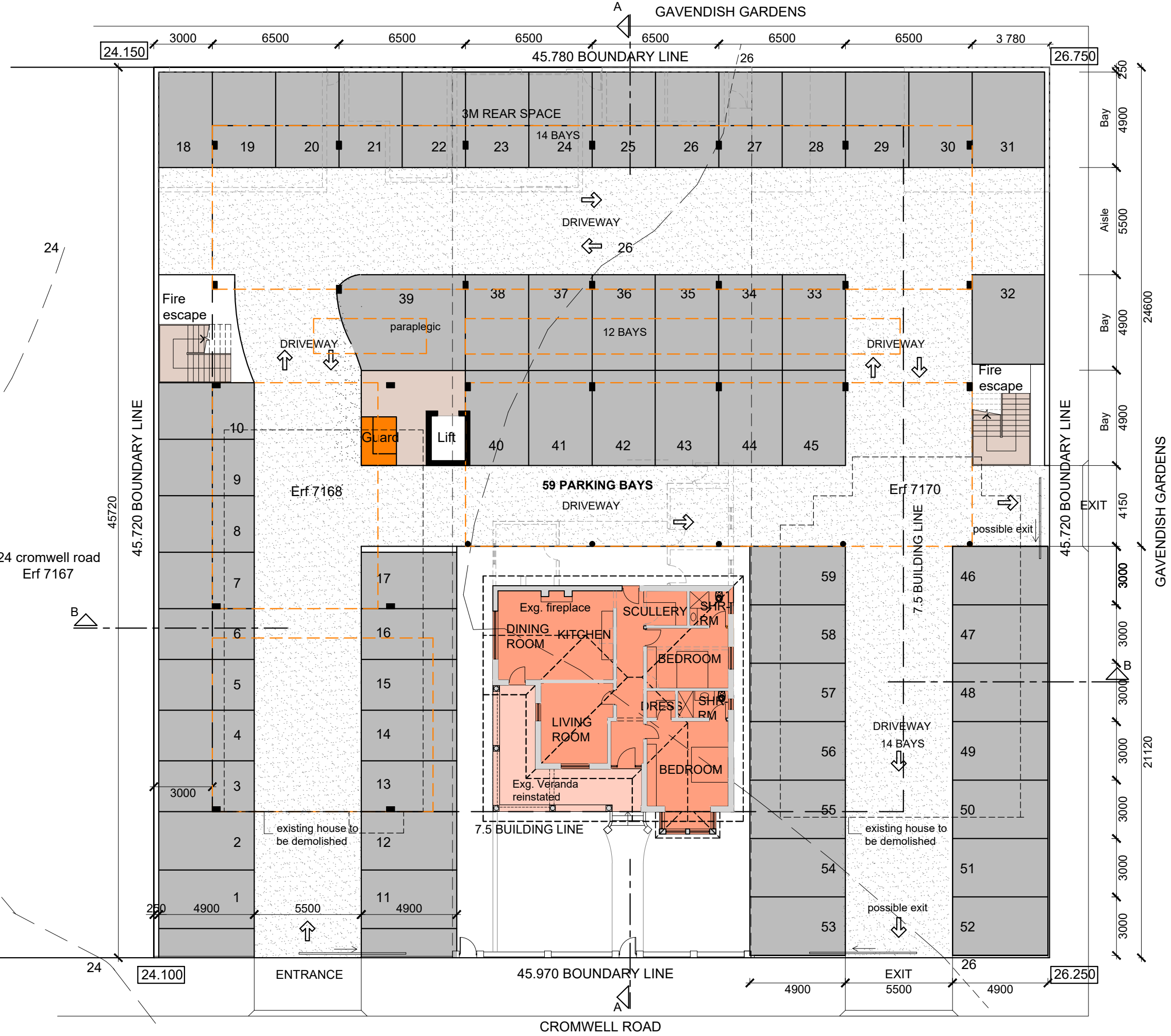
GROUND STOREY PLAN
