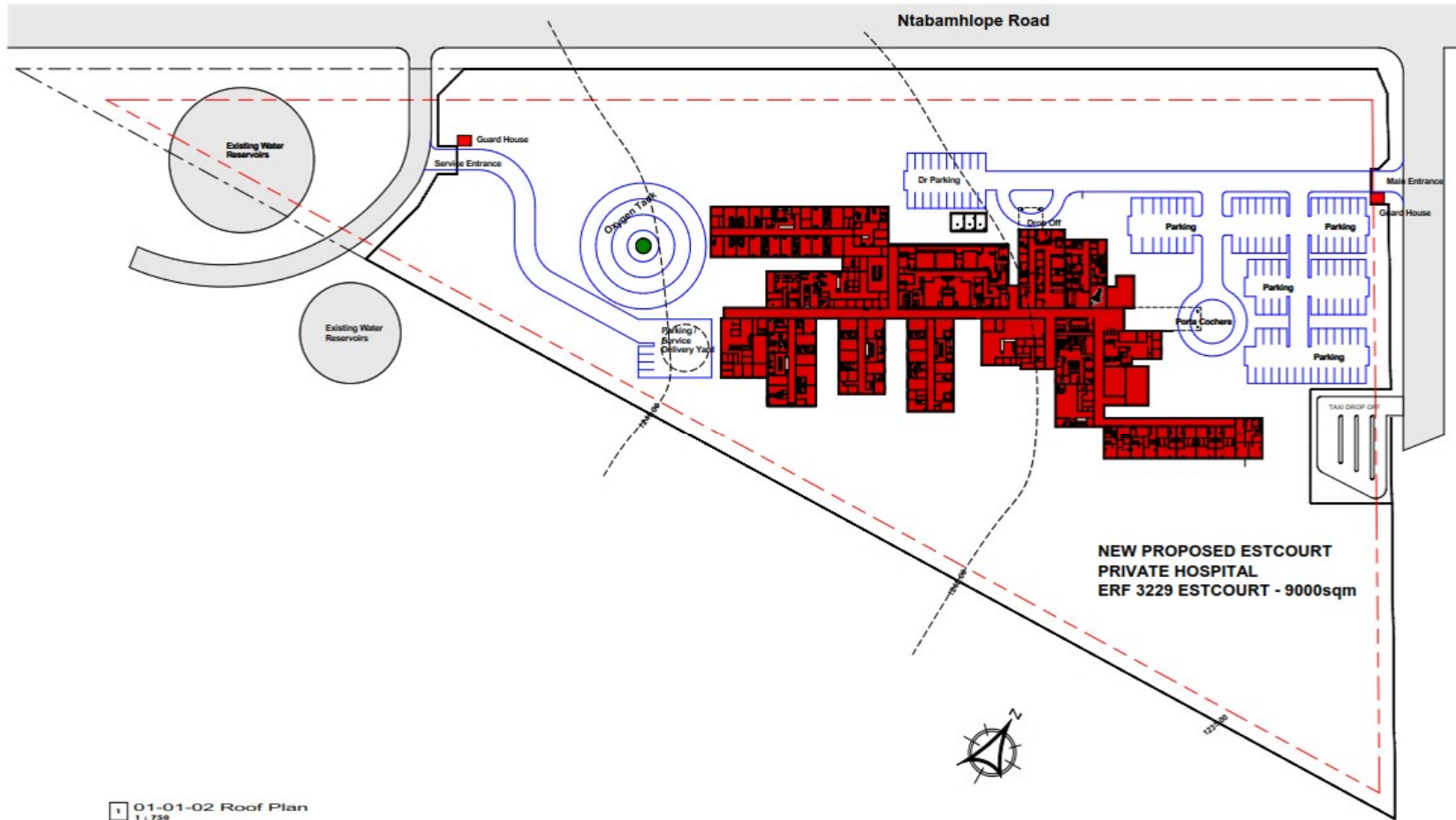
01-01-02 Roof Plan 1:750
