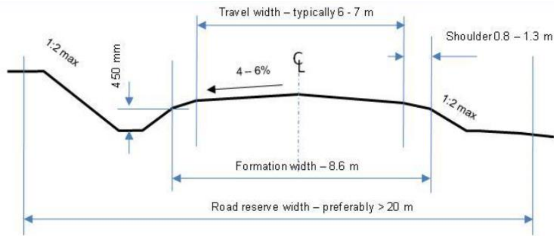
Figure 7:16 Typical Provincial Gravel Road Cross Section
