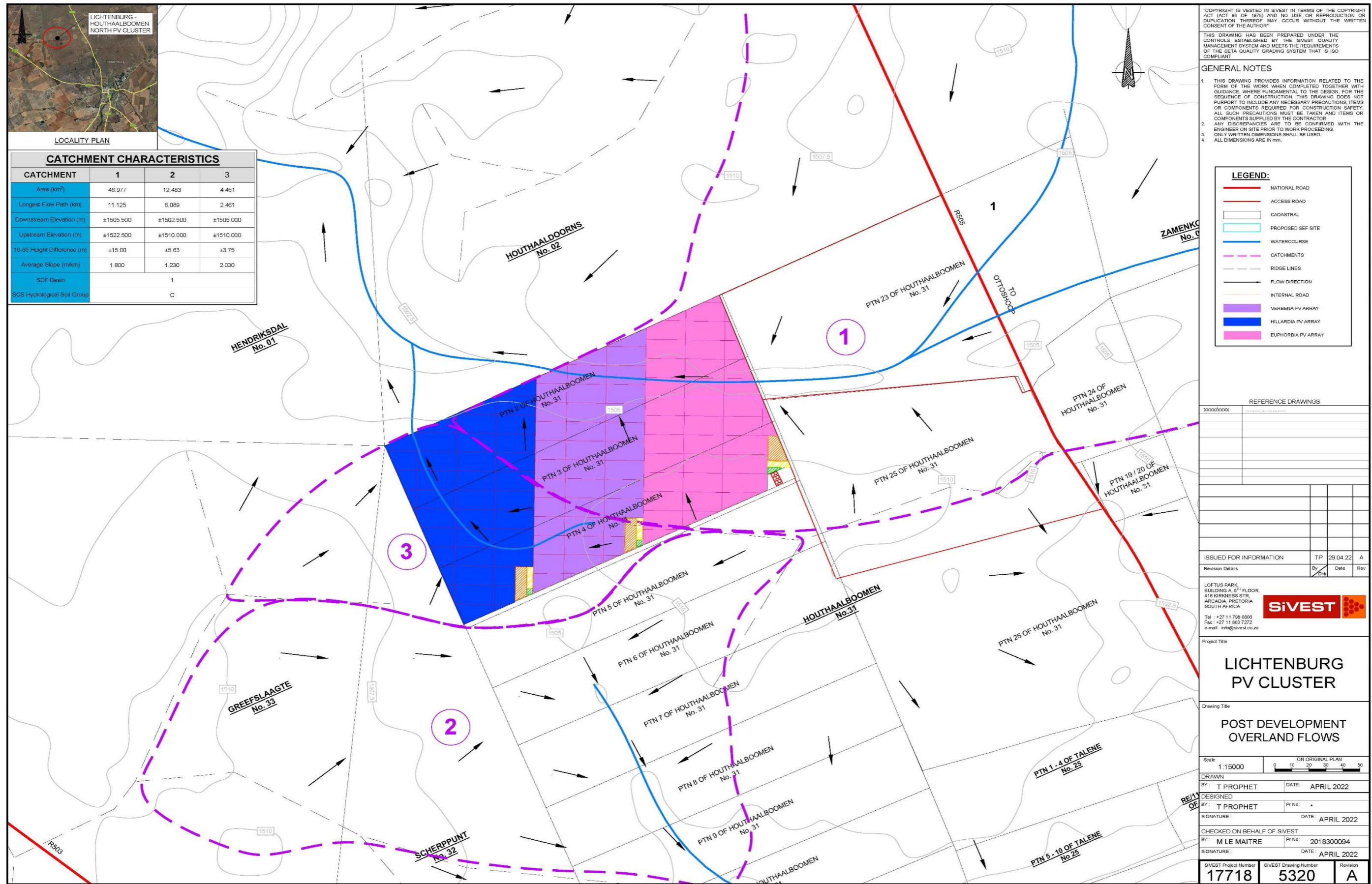
Figure 12:2 Euphorbia PV (Indicated in pink above) – Post-Development Overland Flow
