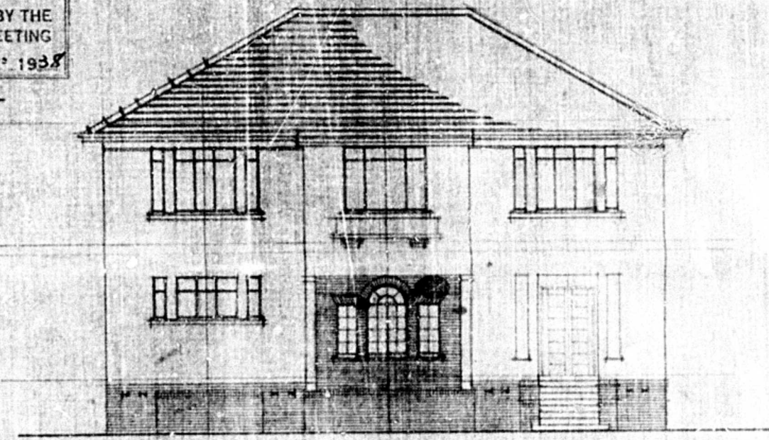
ELEVATION FACING SEA
