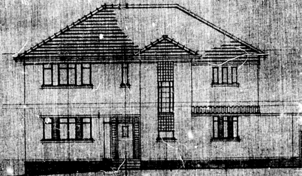
ELEVATION FACING ROAD
