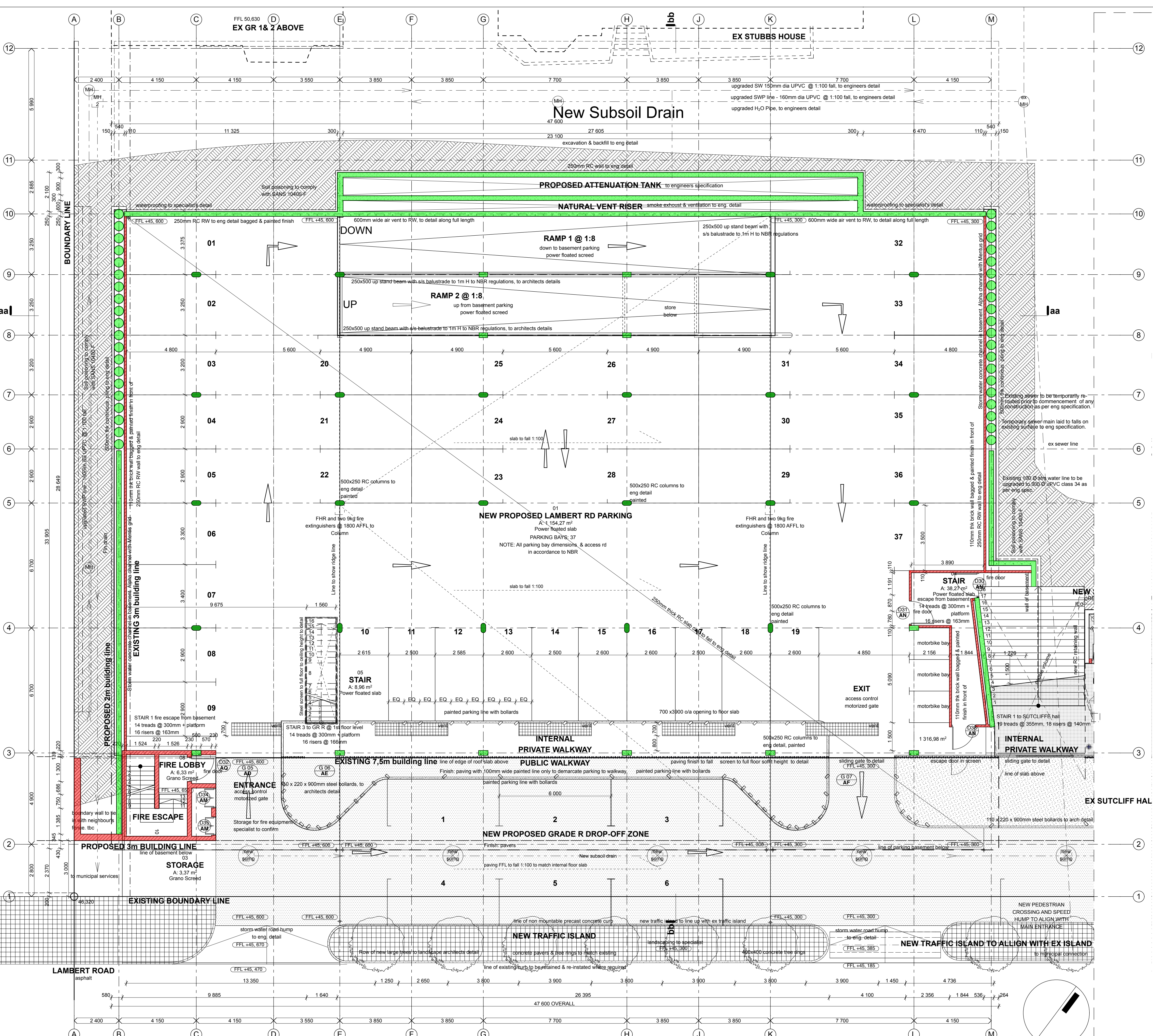
GROUND FLOOR PLAN 1:100
