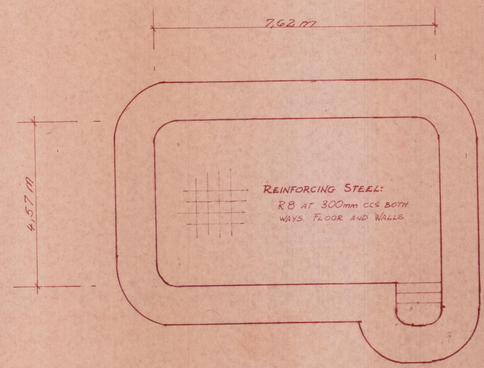
PLAN OF POOL - Area: 35m 2
