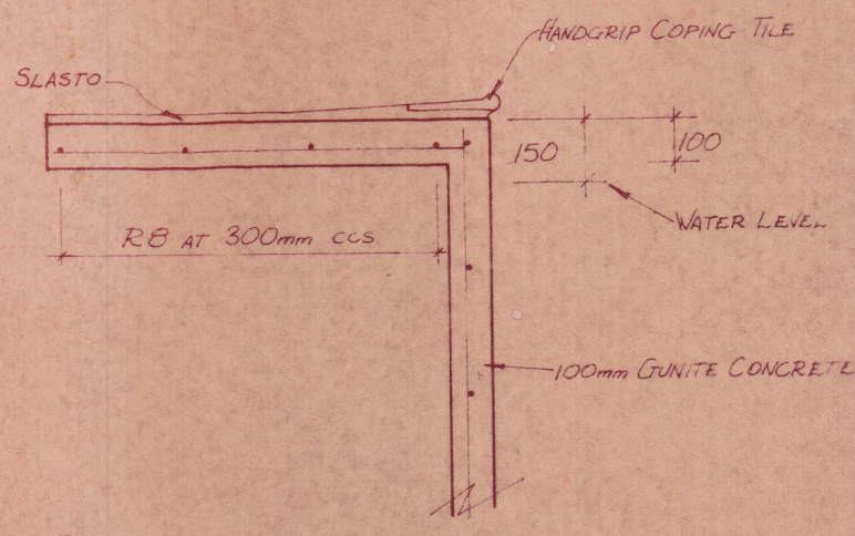
SURROUND BEAM DETAIL - Scale: 1-20
