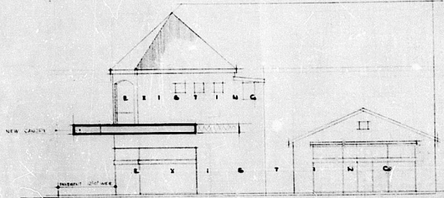
ELEVATION TO DAVILLE STREET
