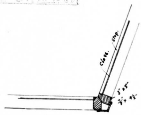
1/4 inch Detail of Corner of Shop Window
