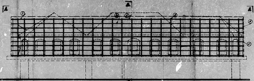
GREY STREET ELEVATION
