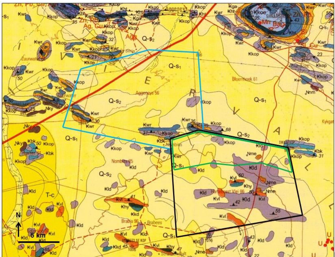
Figure 6-2: Geological Map
