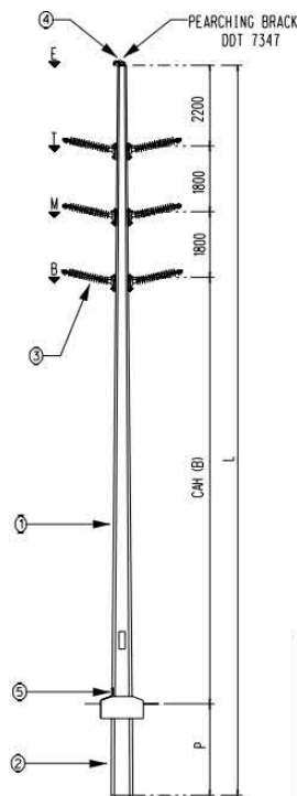
Figure 7-18: Steel / Concrete Monopole Double Circuit Structure
