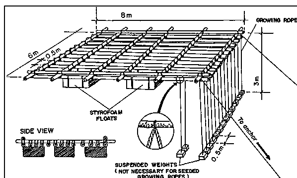
Conceptual drawing of a mussel raft 2
