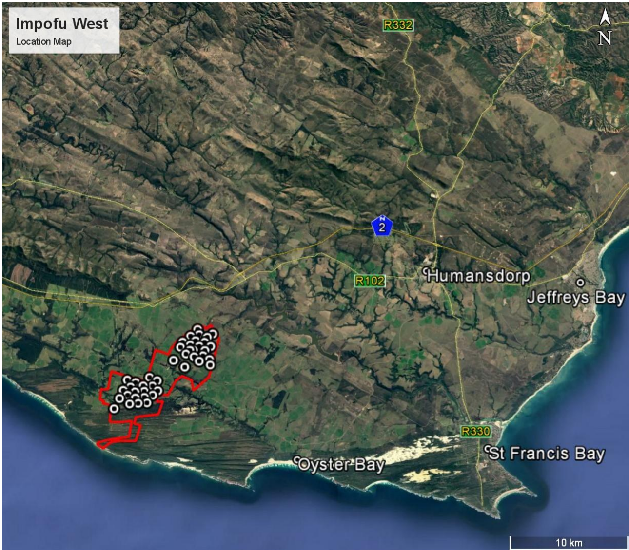
Figure 1. Location map of the proposed development, showing the layout of proposed turbines, west of the town of Humansdorp.
