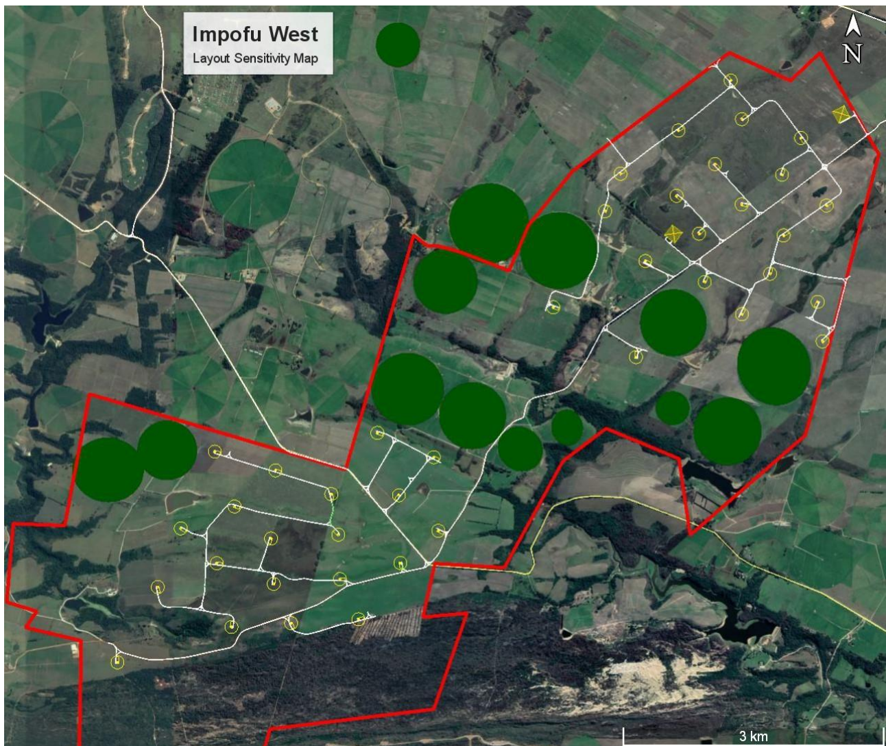
Figure 7. The proposed layout of the Impofu West Wind Farm superimposed on the agricultural No-Go areas.
