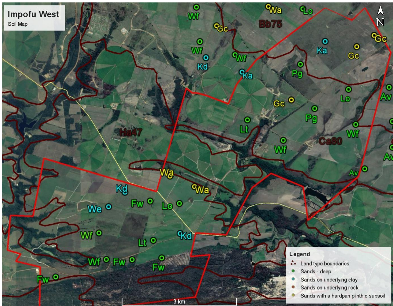
Figure 3. Soil map of development area. Soil form abbreviations indicated on the map are as follows: Fw = Fernwood; Wa = Wasbank; Lo = Longlands; Wf = Witfontein; Kd = Kroonstad; Ka = Katspruit; Gc = Glencoe; Av = Avalon; Pg = Pinegrove; We = Westleigh; Lt = Lamotte. Details of investigated test pits are given in Appendix 1, Table A2.
