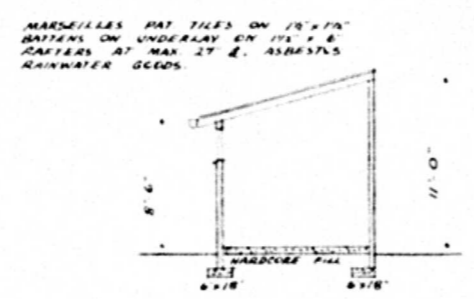
SECT. B-B
