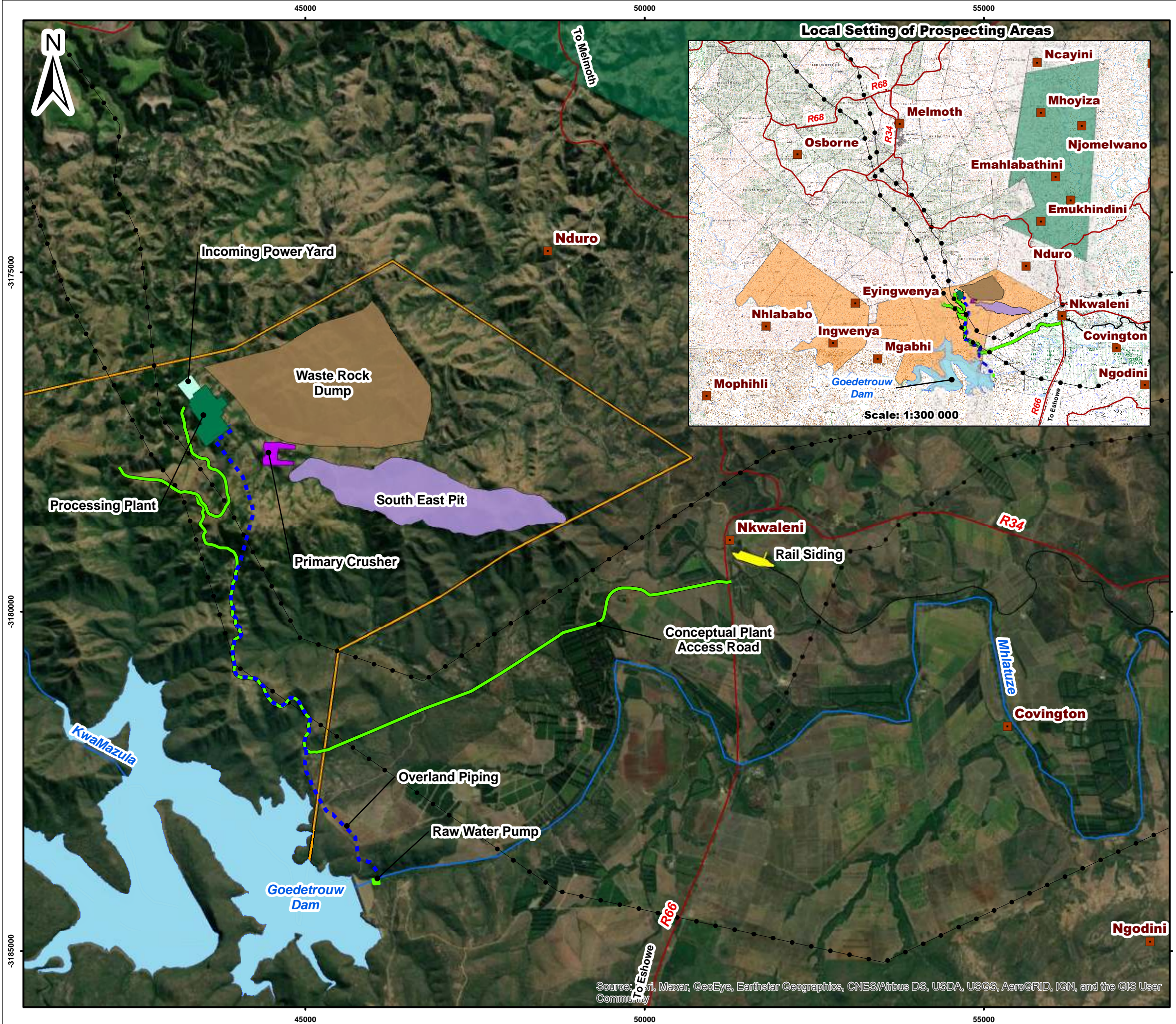
Figure 3-1 Jindal Melmoth Iron Ore Project South Block Proposed Layout
