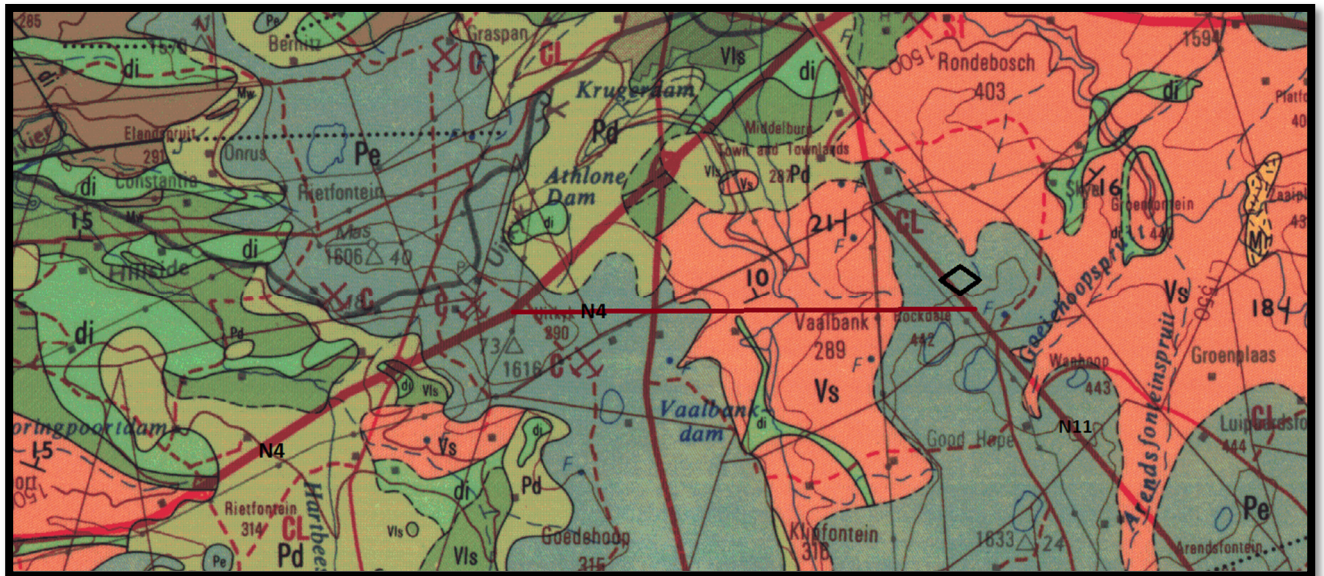
Figure 3: Excerpt of 1:250 000 Geological Map 2630 Mbabane (Walraven 1986).
