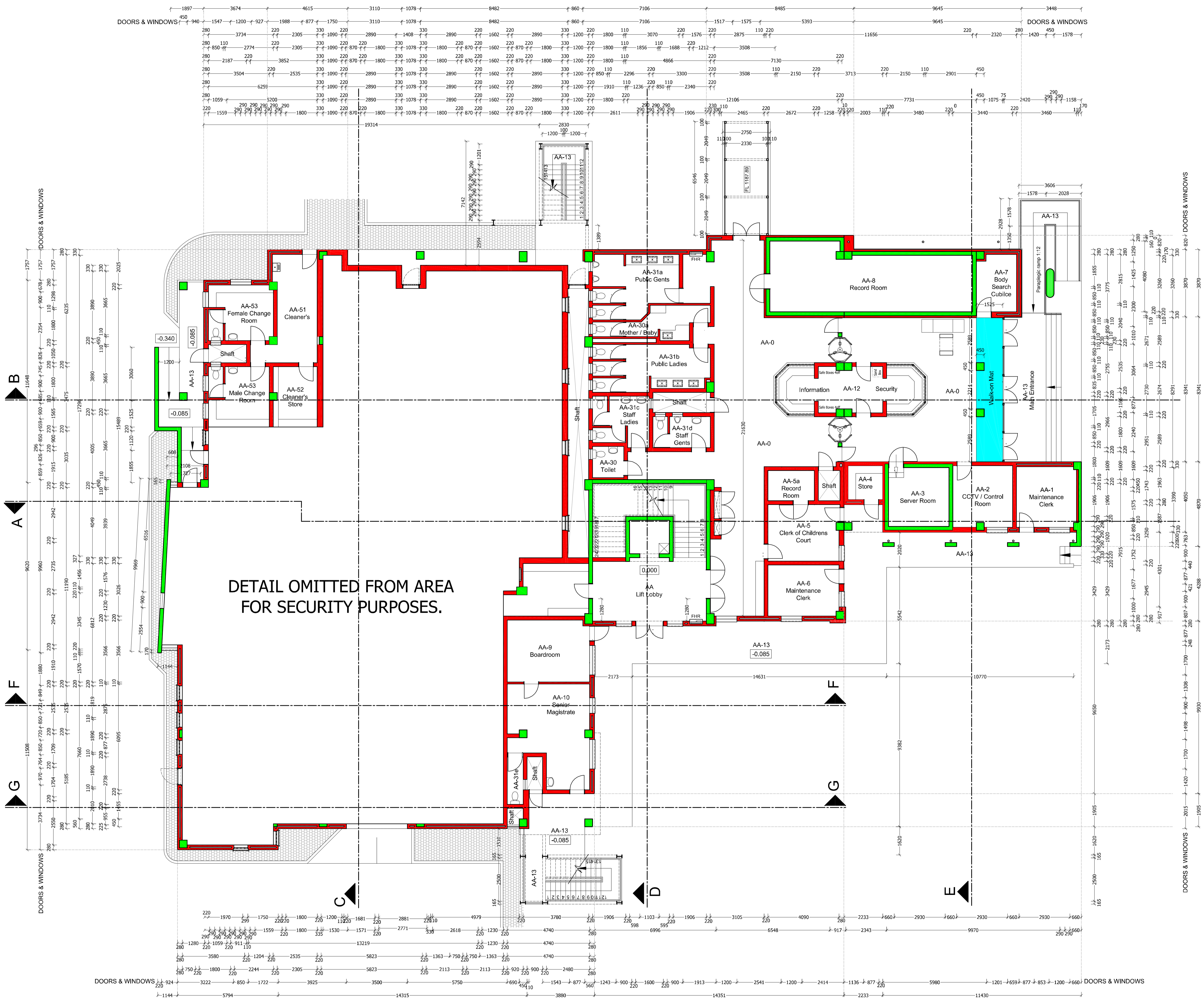
1:100 BLOCK A: GROUND FLOOR DIMENSION PLAN
