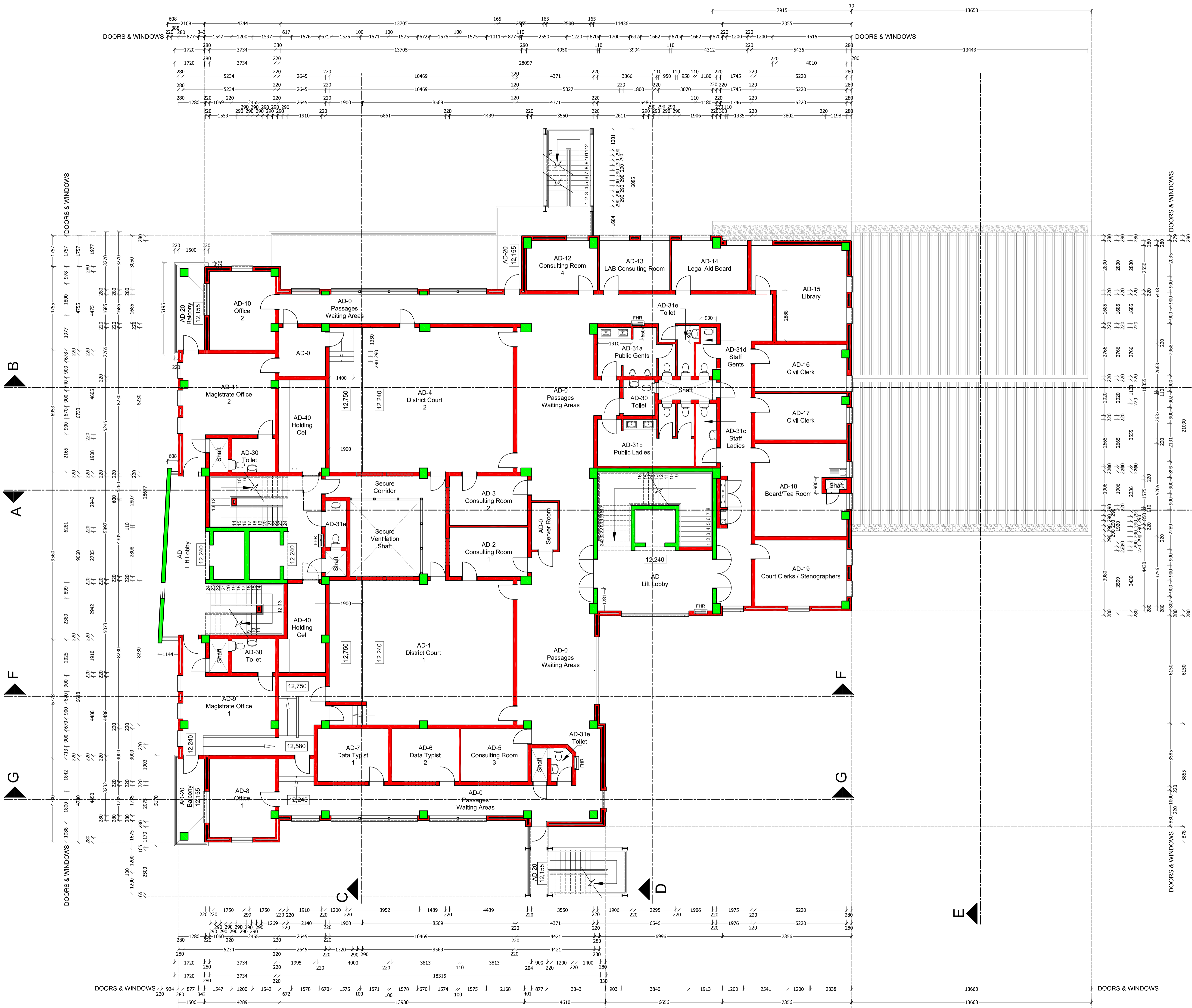
1:100 BLOCK A: THIRD FLOOR DIMENSION PLAN
