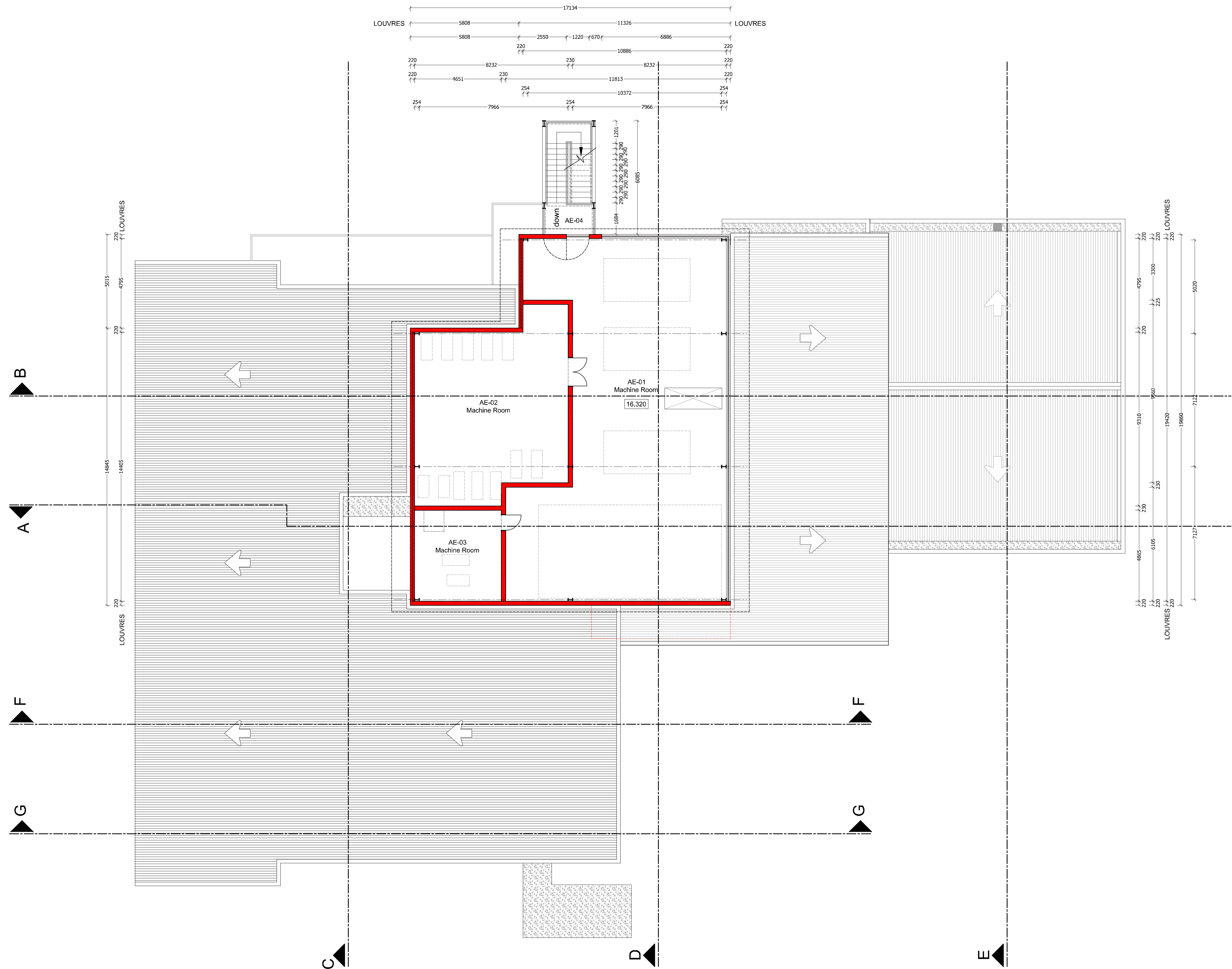
1:100 BLOCK A: FOURTH FLOOR DIMENSION PLAN
