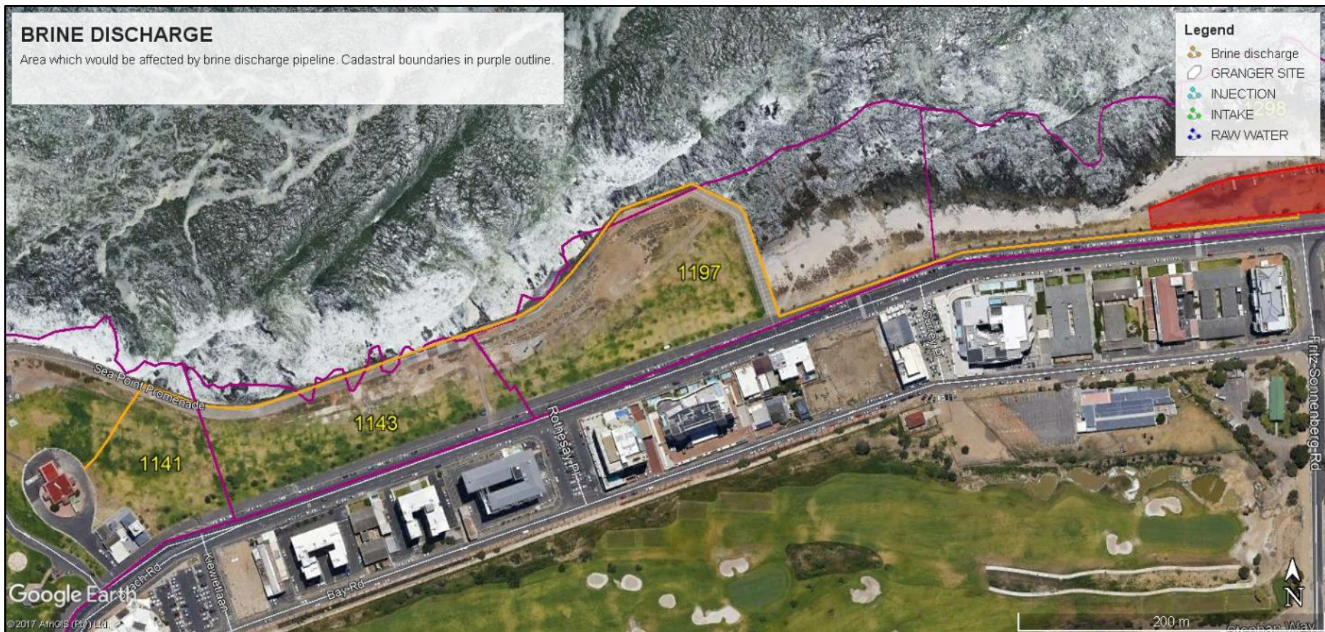
Figure 1.5: Proposed brine discharge pipeline in local context. (Source: Google Earth 2010-01-08 imagery).
