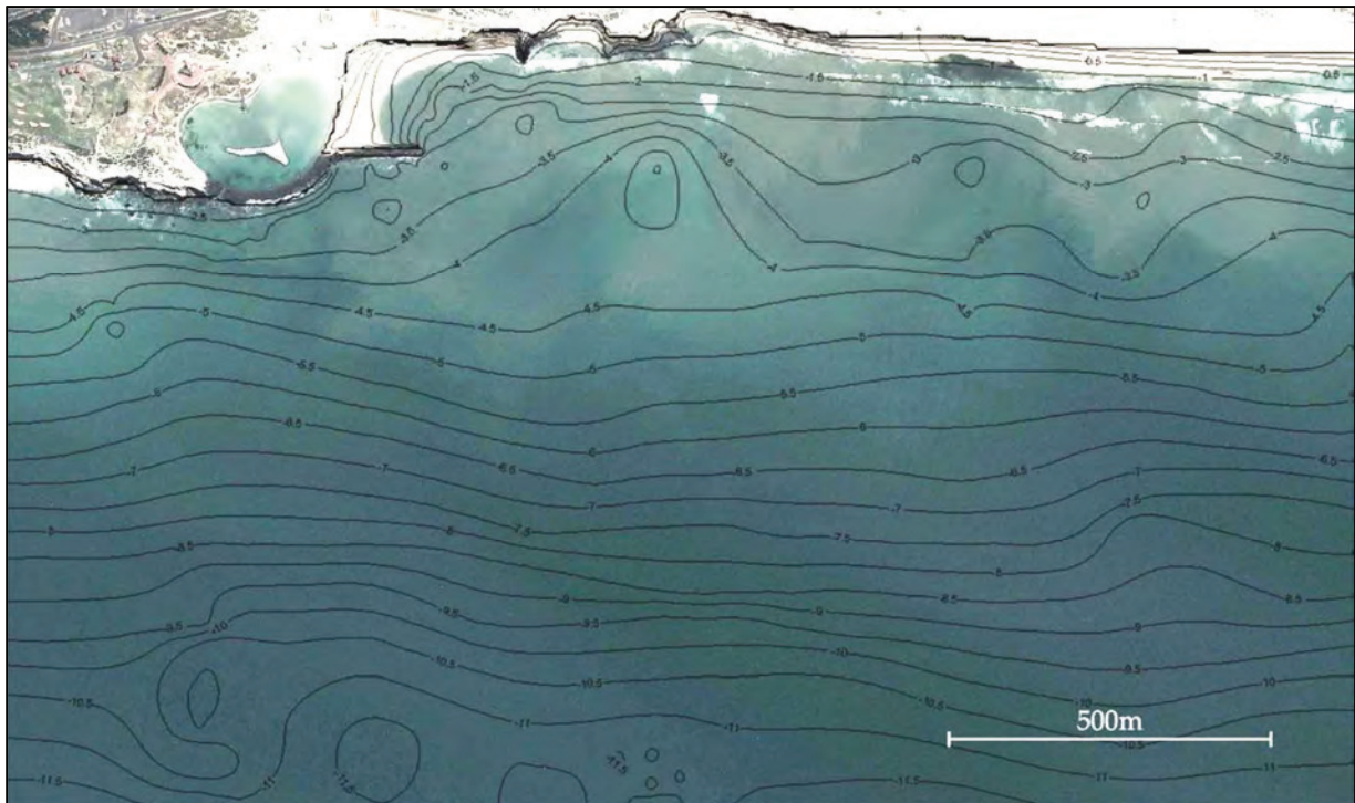
Figure 3A: Bathymetry (m MSL) based on various survey data from the CSIR, dating between 1983 and 1997 (Source: Kistner (2016) 1 )
