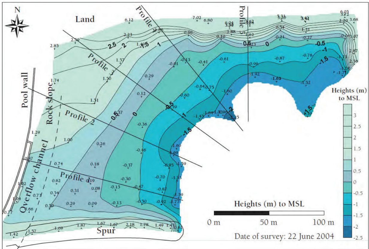
Figure 4A: Measured bathymetry east of the tidal pool (June 2014), referenced to MSL (Source: Theron and Schoonees 2007 2 )
