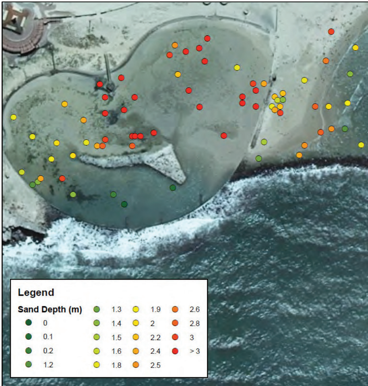
Figure 7A: Jet probing near Monwabisi
