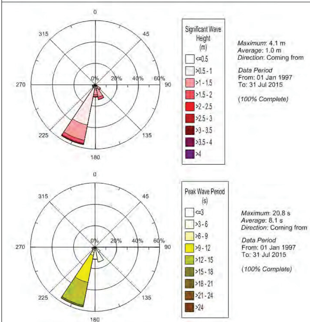
Figure 9A: Indicative annual wave rose for Position 1, Monwabisi
