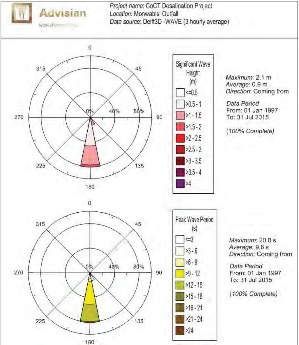
Figure 10A: Indicative annual wave rose for Position 2, Monwabisi
