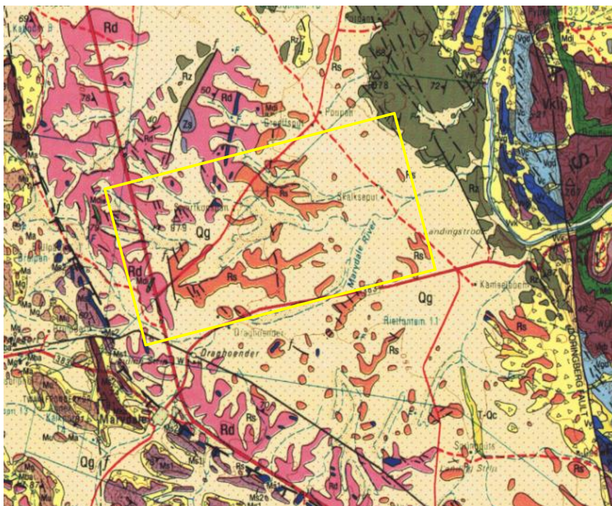
Figure 2: Geological map of the area around the Farms Rietfontein 11 and Farm 20 with the prospecting area indicated within the yellow rectangle. Abbreviations of the rock types are explained in Table 2. Map enlarged from the Geological Survey 1: 250 000 map 2922 Prieska.
