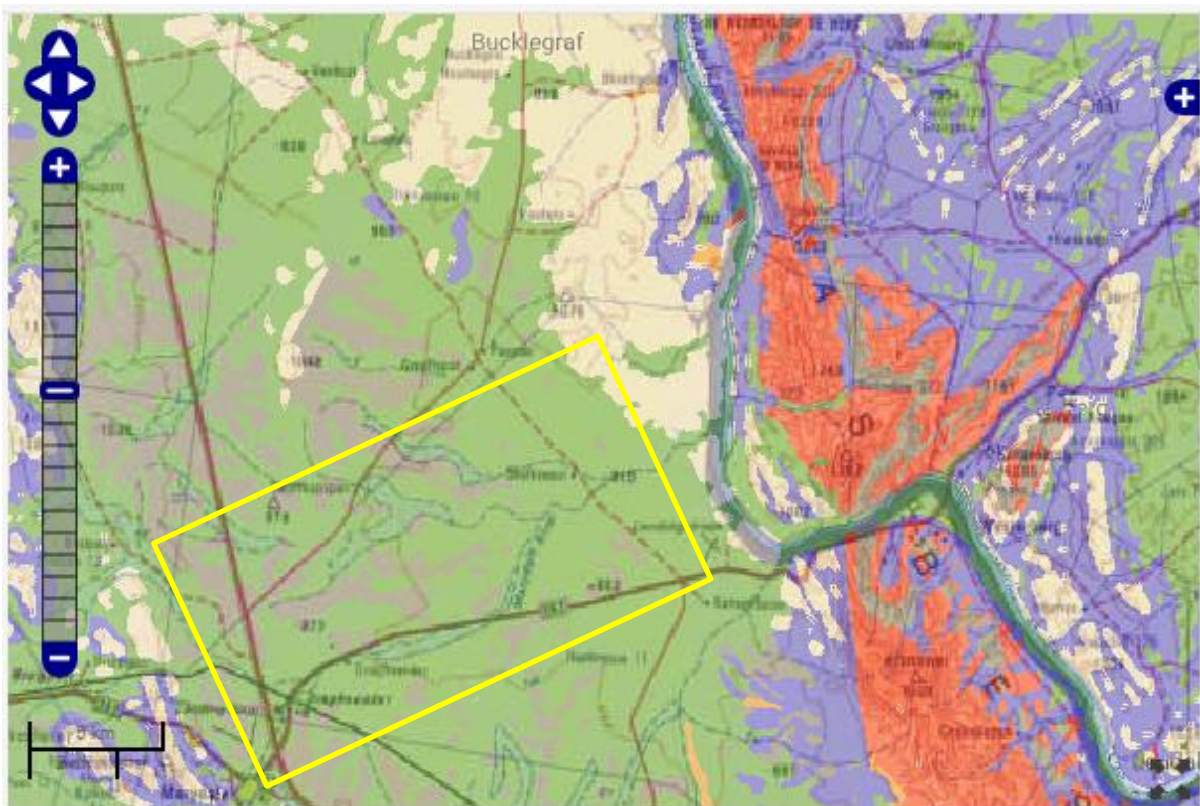
Figure 3: SAHRIS palaeosensitivity map for the site for the proposed PRA on Farms Rietfontein 11 and Farm 20 (project 3) shown within the yellow rectangle. Background
