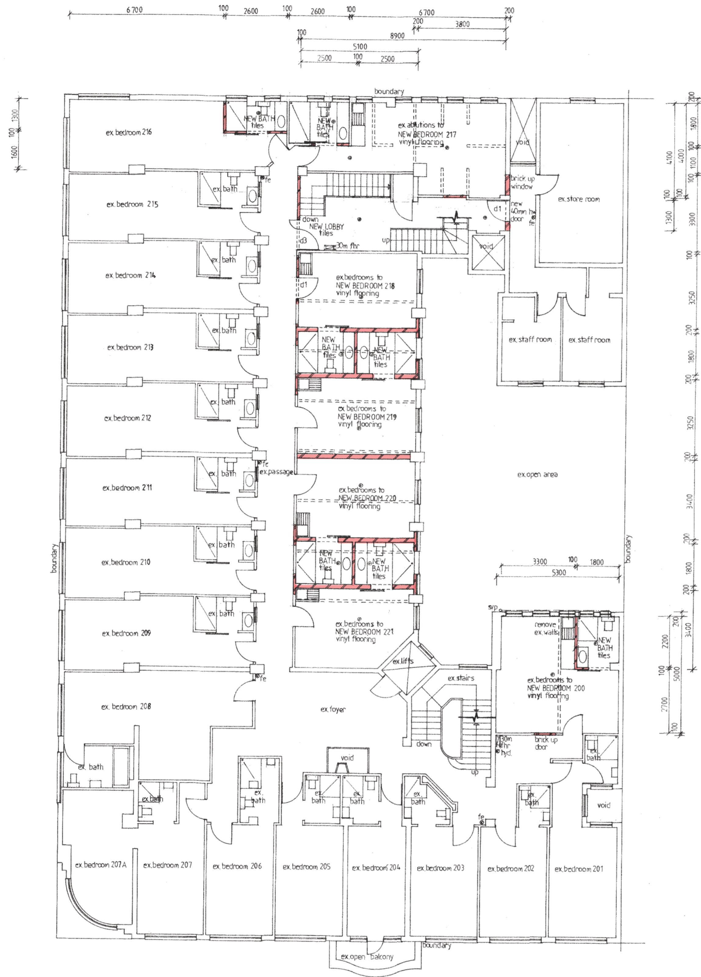
SECOND STOREY PLAN (1:100)
