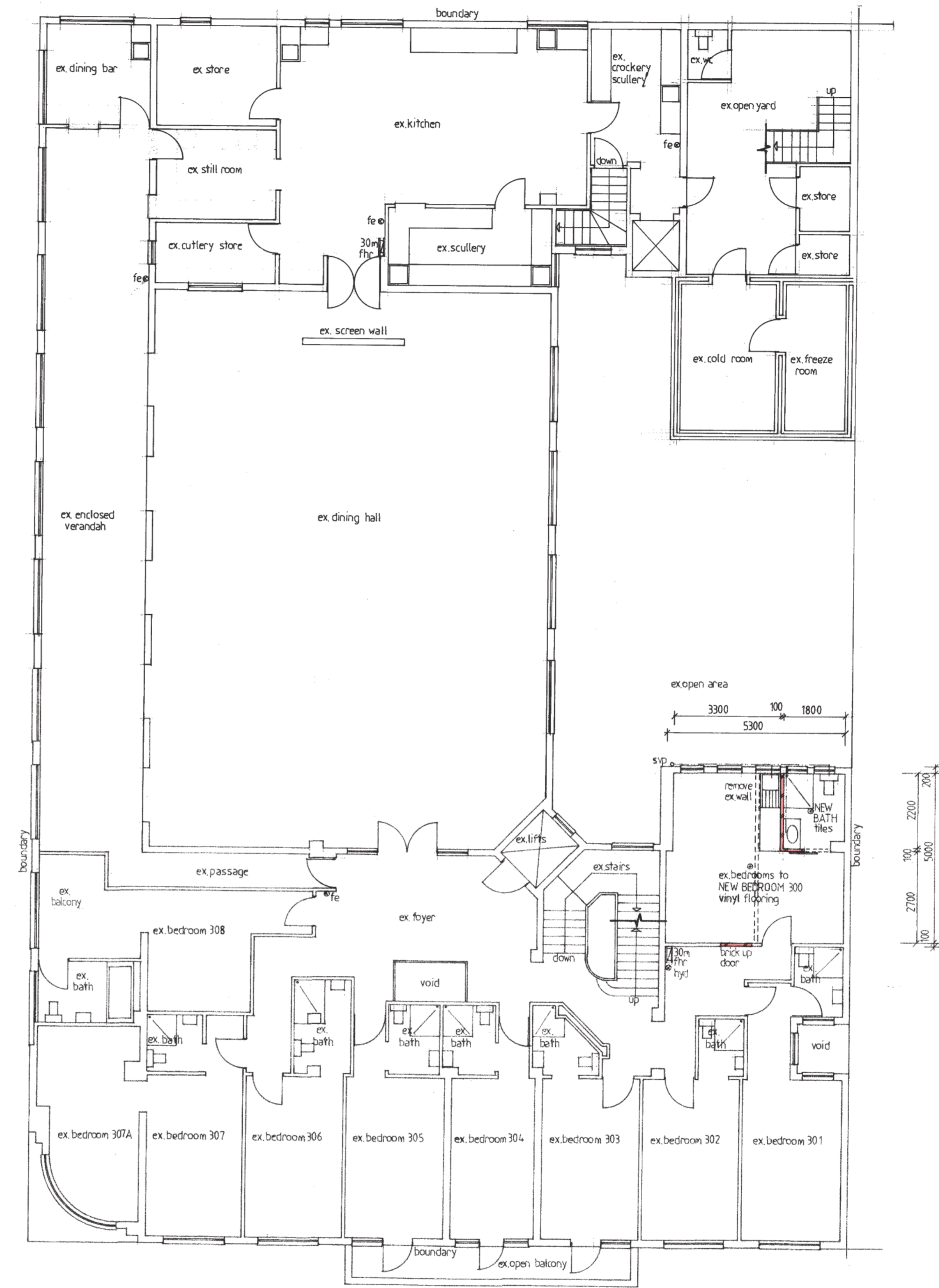
THIRD STOREY PLAN (1:100)
