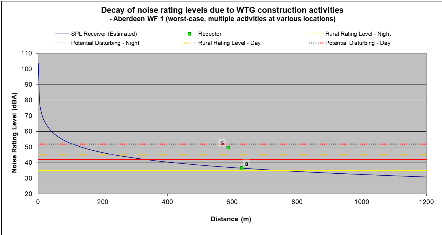
Figure 9-3: Projected conceptual construction noise levels for the proposed Aberdeen WF 1
