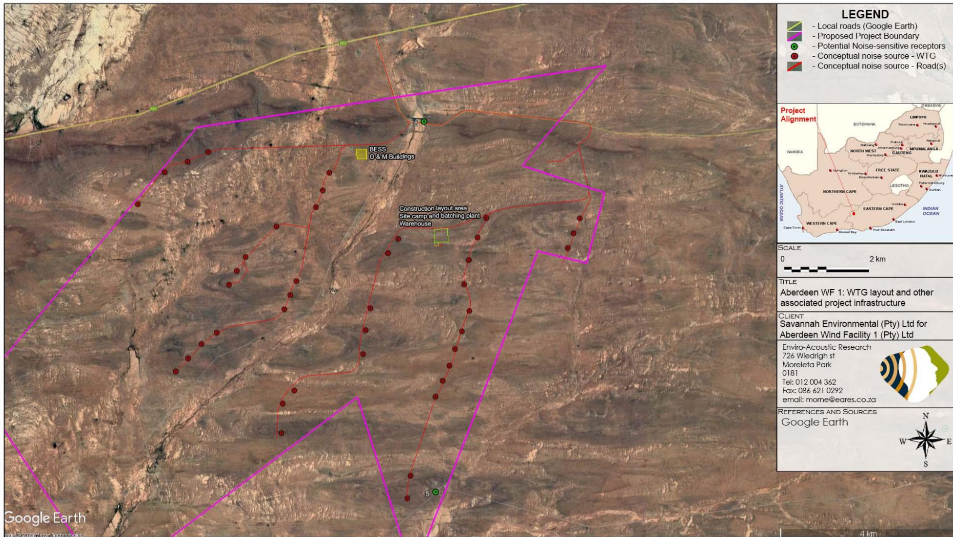
Figure 9-1: WTG locations and associated infrastructure for the proposed Aberdeen WF 1
