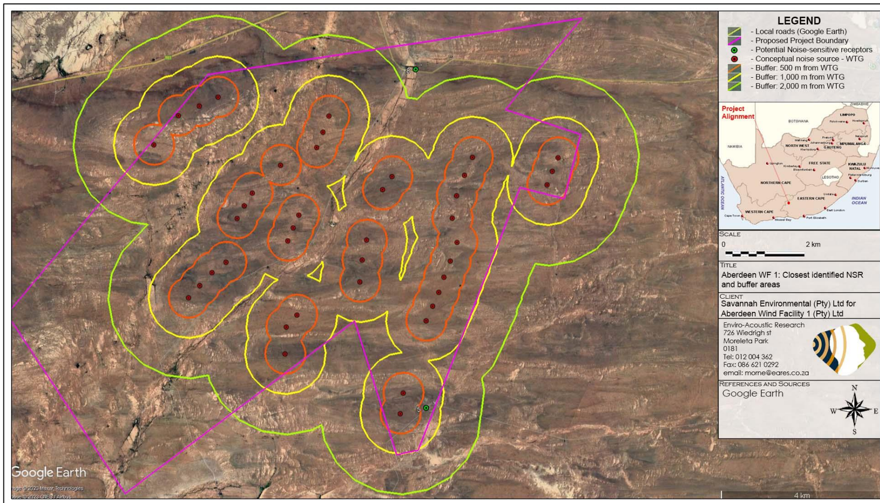
Figure 2-2: Study area and potential noise-sensitive receptors close to Aberdeen WF 1
