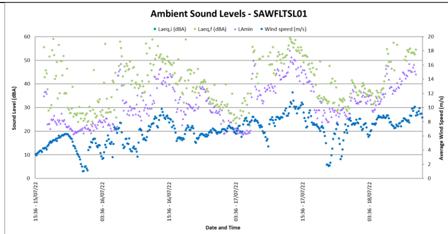
Figure 4-4: Ambient Sound Levels at SAWFLTSL01
