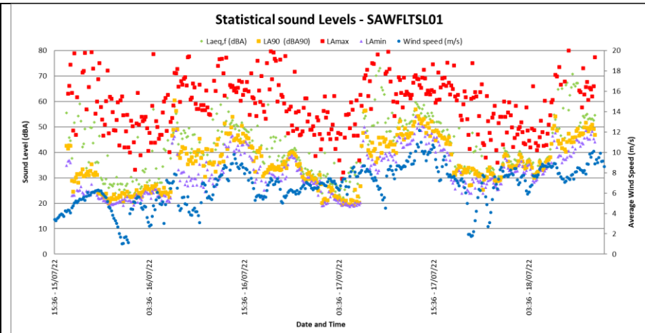
Figure 4-5: Maximum, minimum and Statistical sound levels at SAWFLTSL01
