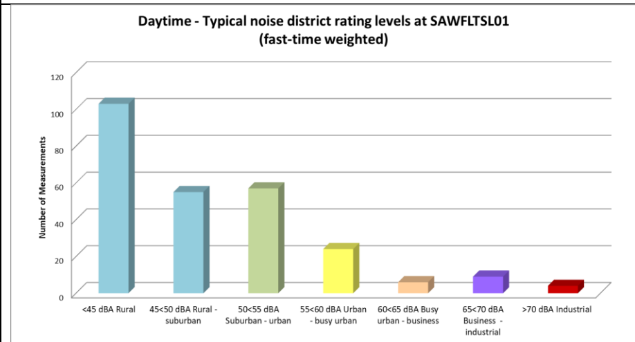
Figure 4-7: Classification of daytime measurements in typical noise districts at SAWFLTSL01
